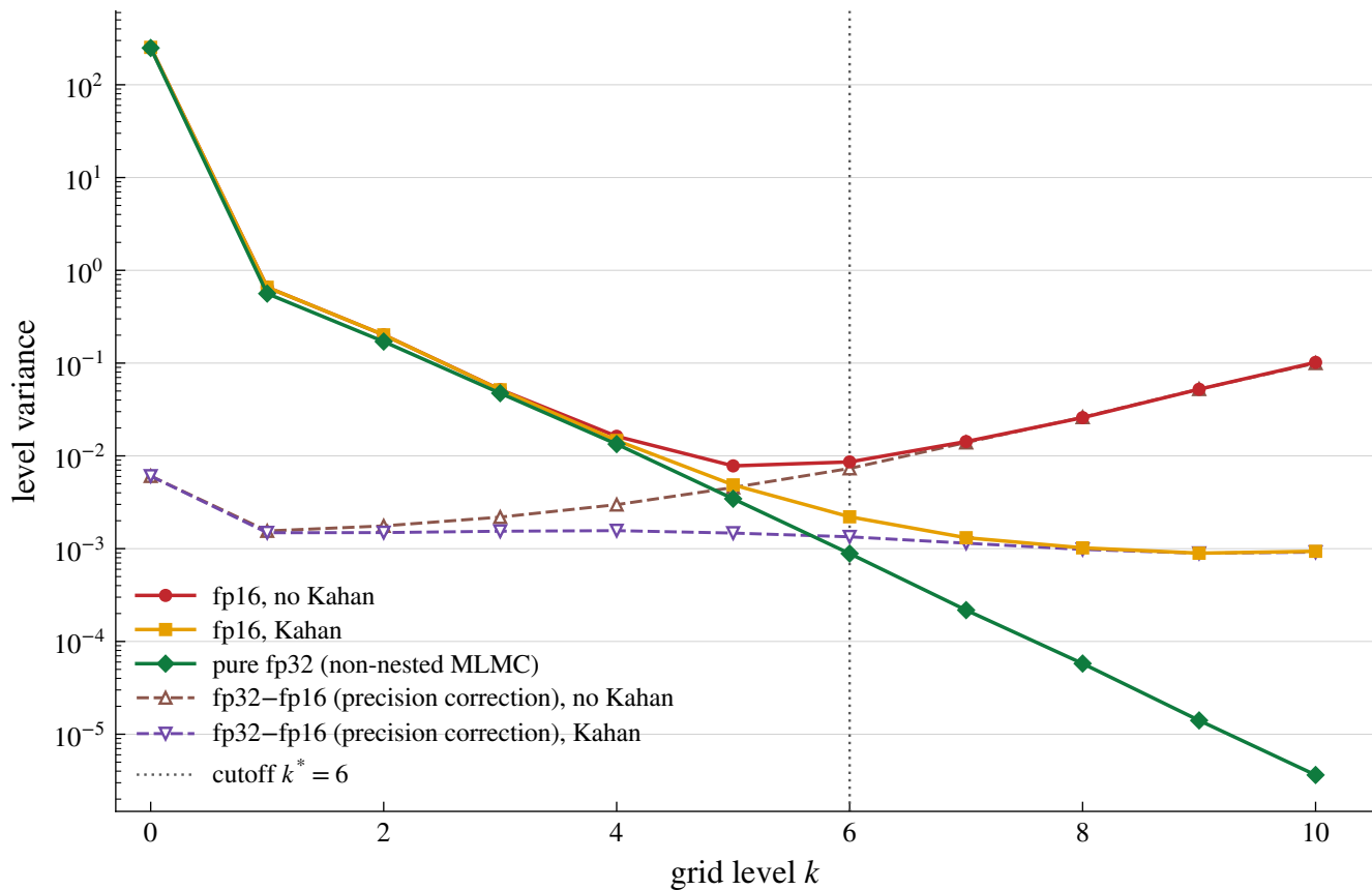
Basket European: AVX-512 fp16/fp32 precision comparison ( N = 20,000 )
