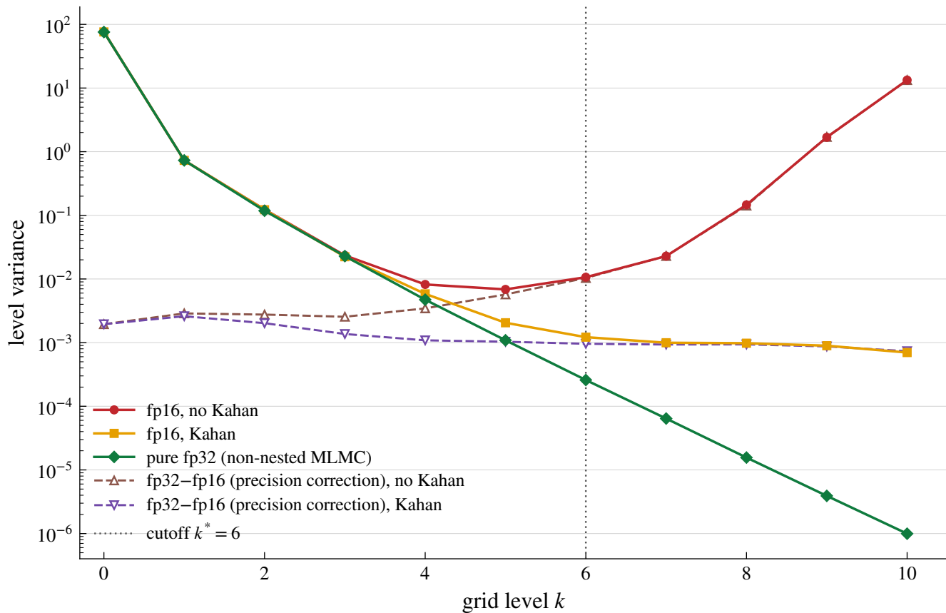
Basket Asian: AVX-512 fp16/fp32 precision comparison ( N = 20,000 )
