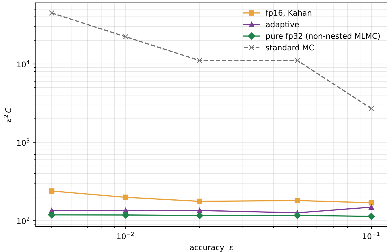
Scalar Asian: cost complexity
