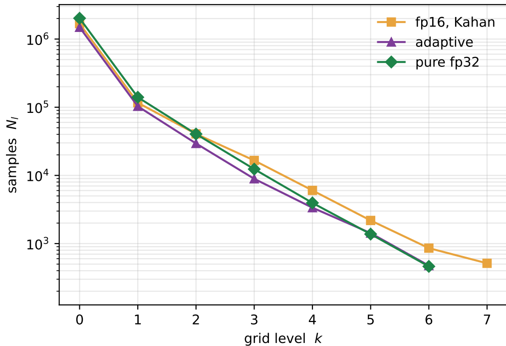
Milstein correction (even l = 2k )
