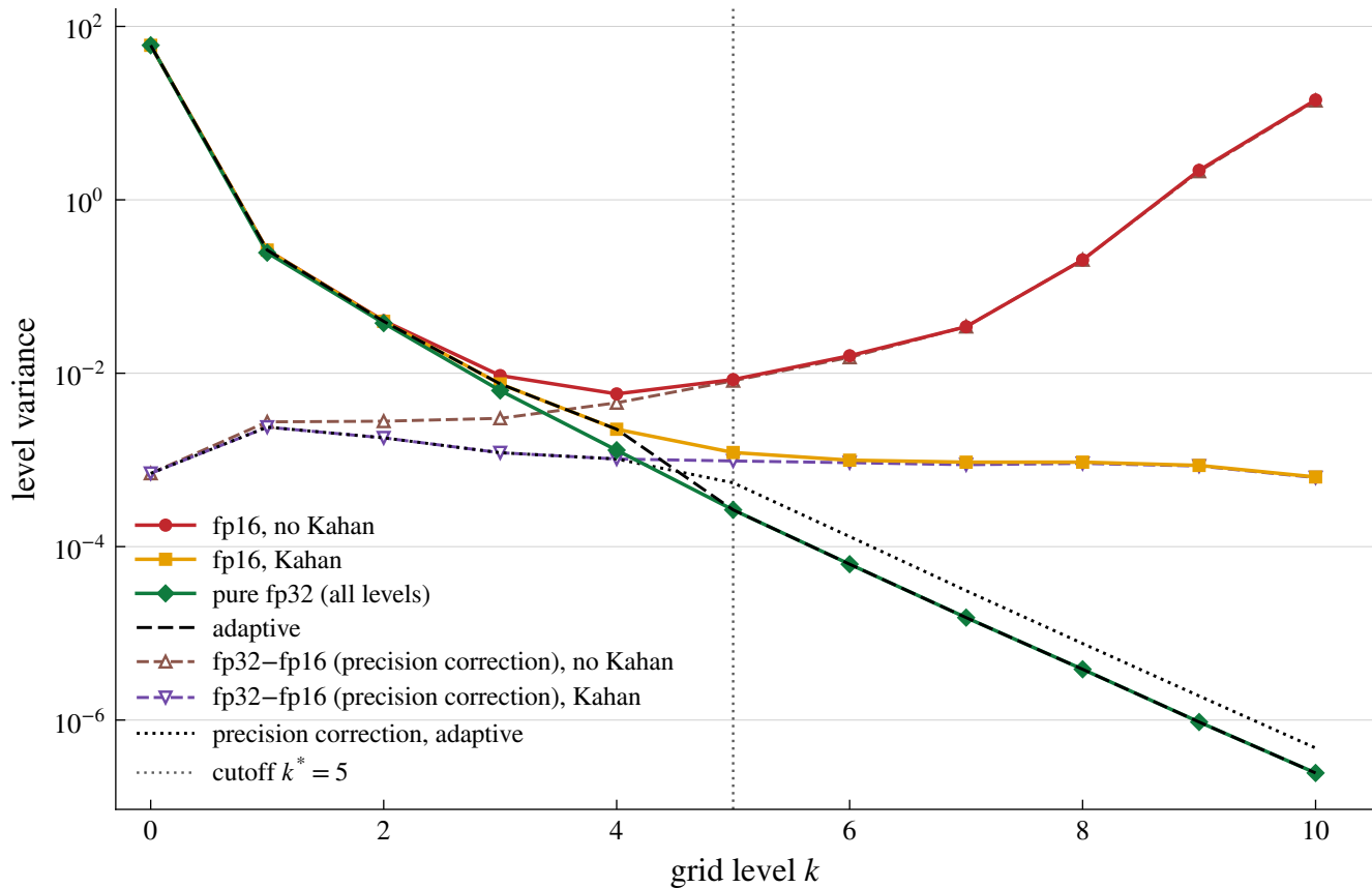
Scalar Asian: AVX-512 fp16/fp32 precision comparison ( N = 20,000 )
