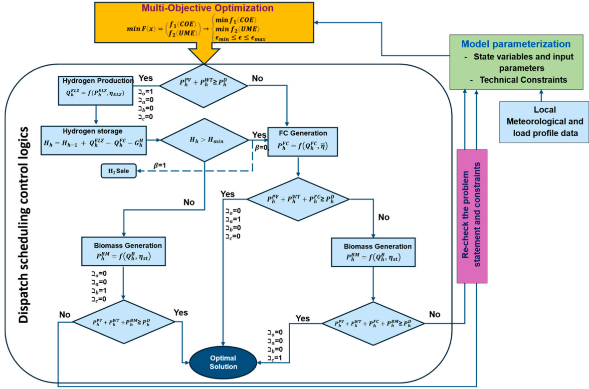
Fig. 4. Overall structure of the dispatch model developed in this study with detailed unit commitment strategy.
