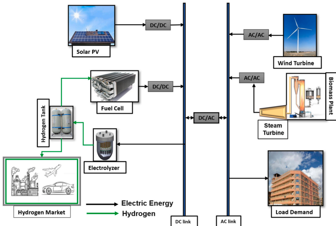
Fig. 1. Schematic diagram of the Proposed H2-HRES in this study.
