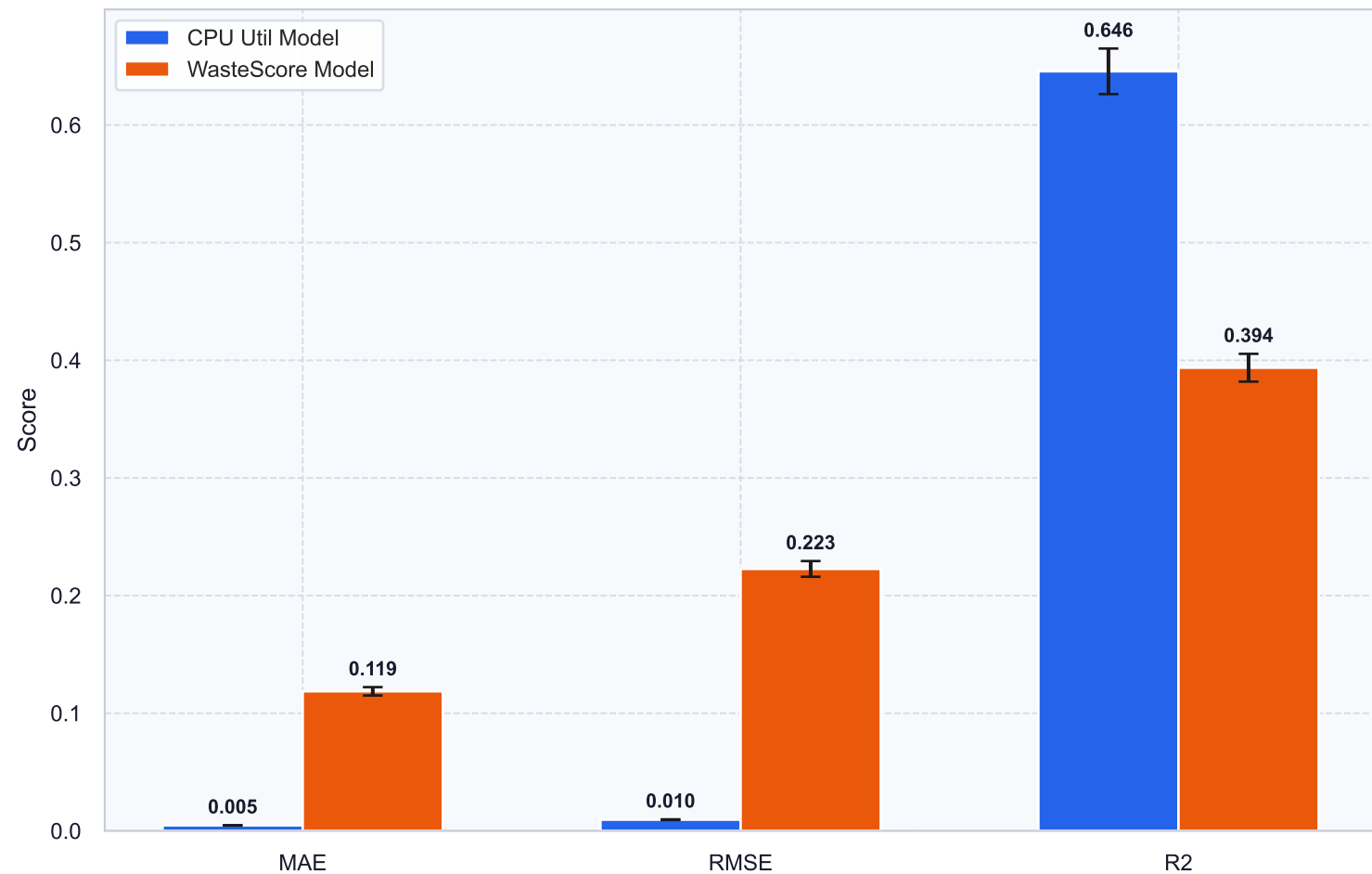
Model Performance Metrics (with 95% CI)
