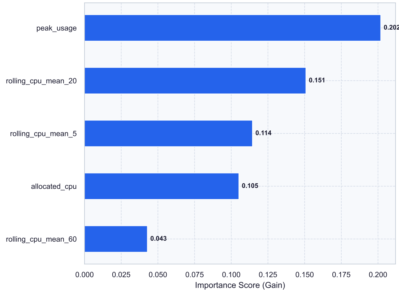
CPU Utilisation Model — Top-5 Features
