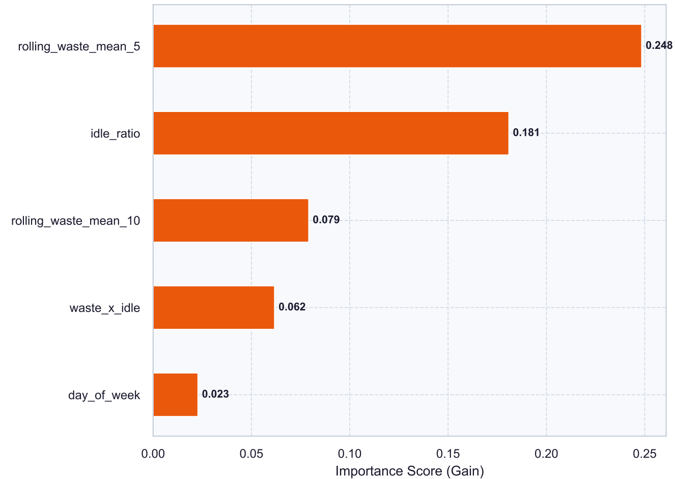
WasteScore Model — Top-5 Features
