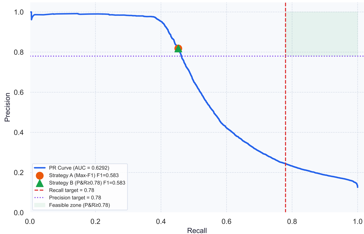
Precision-Recall Curve — Ensemble Classifier
