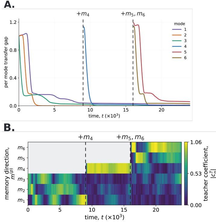
Fig 5. Staged memory acquisition renews reactivation and memory transfer. A 50-unit linear teacher-student network was followed through one continuous run during the transfer of 6 random memory patterns. The teacher initially stored m_1 , m_2 , and m_3 ; it acquired m_4 at t = 9000 and acquired m_5 and m_6 together at t = 16000 through interleaved teacher training on the whole corpus. Coupled intrinsic dynamics resumed after each acquisition without resetting student activity or recurrent weights. Dashed lines mark the acquisition events. A , Per-mode transfer gaps during the simulation. Previously transferred modes keep a small error, whereas each newly supported mode introduces a large transfer gap that subsequently decreases. B , Memory coefficient magnitudes |c_p^T(t)| , which measure the contribution of each stored pattern m^{(p)} to teacher activity x_T(t) (Methods). Low values mean that the teacher does not reactivate the corresponding memory, whereas high values indicate strong reactivation. Newly added memories initially receive a stronger reactivation drive. As transfer progresses, this drive decreases.
