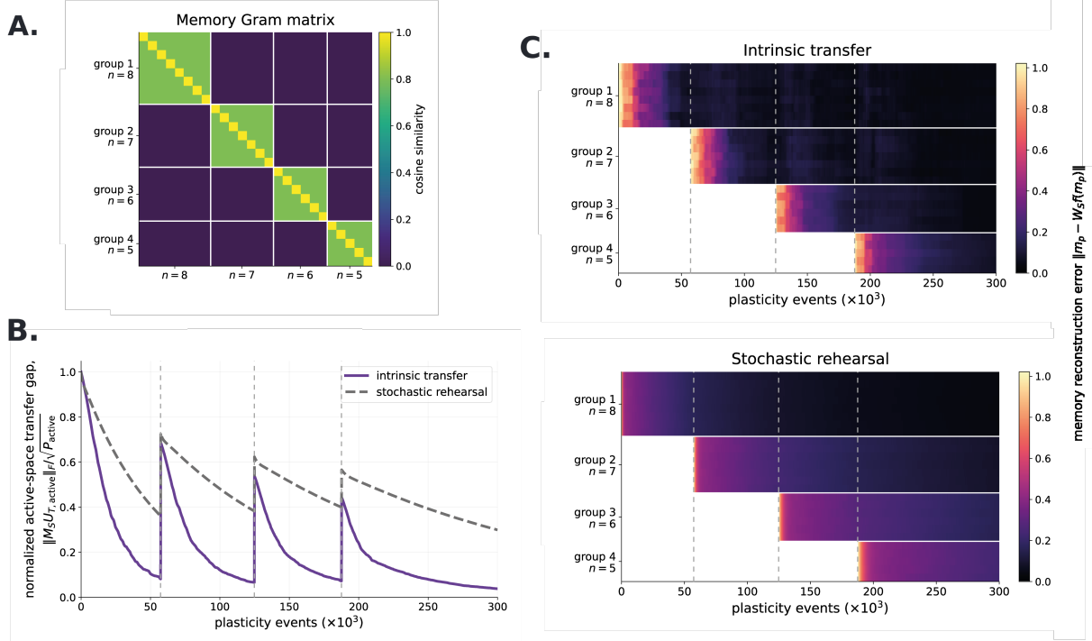
Fig 8. Continuous addition of correlated memory groups increases the intrinsic-transfer advantage. As in the staged-acquisition experiment in Fig. 5, memories were added during one uninterrupted transfer run by retraining the teacher on the enlarged corpus containing both the previously stored and newly introduced memories. The students retained their activity and recurrent weights across acquisition events. The corpus contained 26 memories arranged into four mutually orthogonal groups of 8, 7, 6, and 5 memories, with exact within-group cosine similarity \rho = 0.80 . Group 1 was present initially, and groups 2, 3, and 4 were introduced after 57,300, 124,800, and 187,600 plasticity events, respectively. Dashed vertical lines mark these acquisitions. A , Memory Gram matrix for the complete corpus. B , Normalized active-space transfer gap \|M_S U_{T, \text{active}}\|_F / \sqrt{P_{\text{active}}} for intrinsic transfer (purple solid curve) and stochastic rehearsal (gray dashed curve). Here, U_{T, \text{active}} is an orthonormal basis of the memory space supported by the teacher at that stage, and P_{\text{active}} is the number of memories then available. Each acquisition expands the measured space and produces an upward jump in the gap. Intrinsic transfer reduces the gap faster during every stage. C , Reconstruction errors for individual memories during intrinsic transfer (top) and stochastic rehearsal (bottom). White cells denote memories that have not yet been added to the active corpus. Once a group becomes active, its reconstruction errors decrease faster under intrinsic transfer, consistent with redistribution being directed toward the newly unsupported content.
