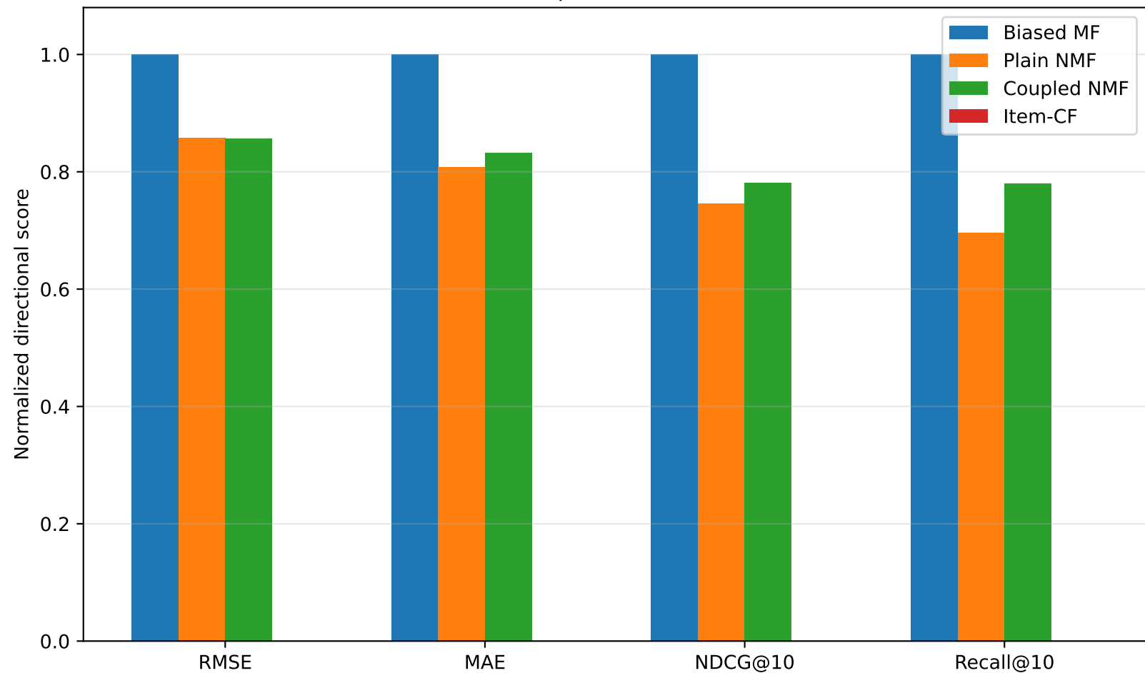
Overall benchmark comparison on MovieLens latest-small
