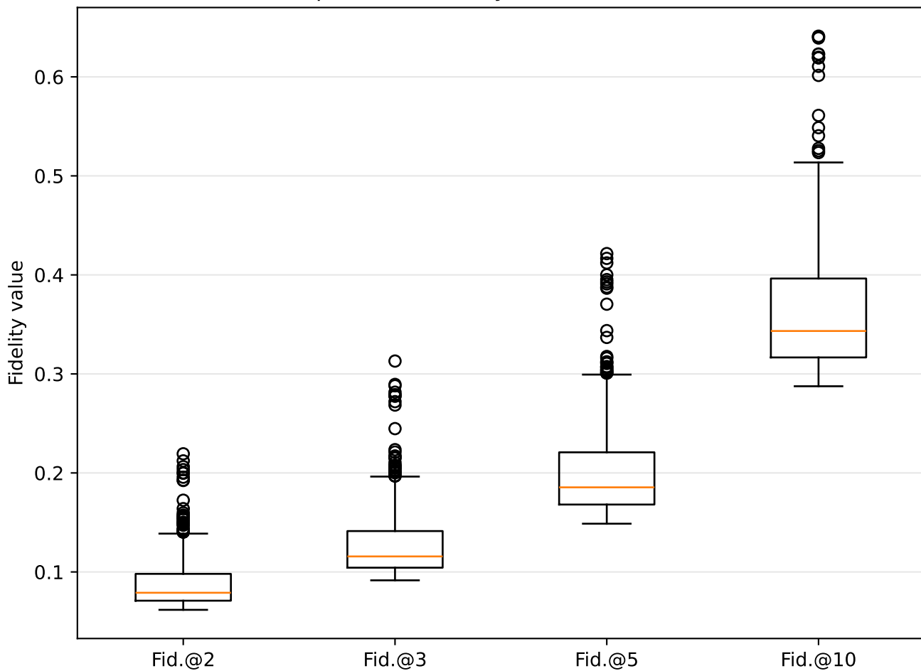
Distribution of explanation fidelity over recommendation instances
