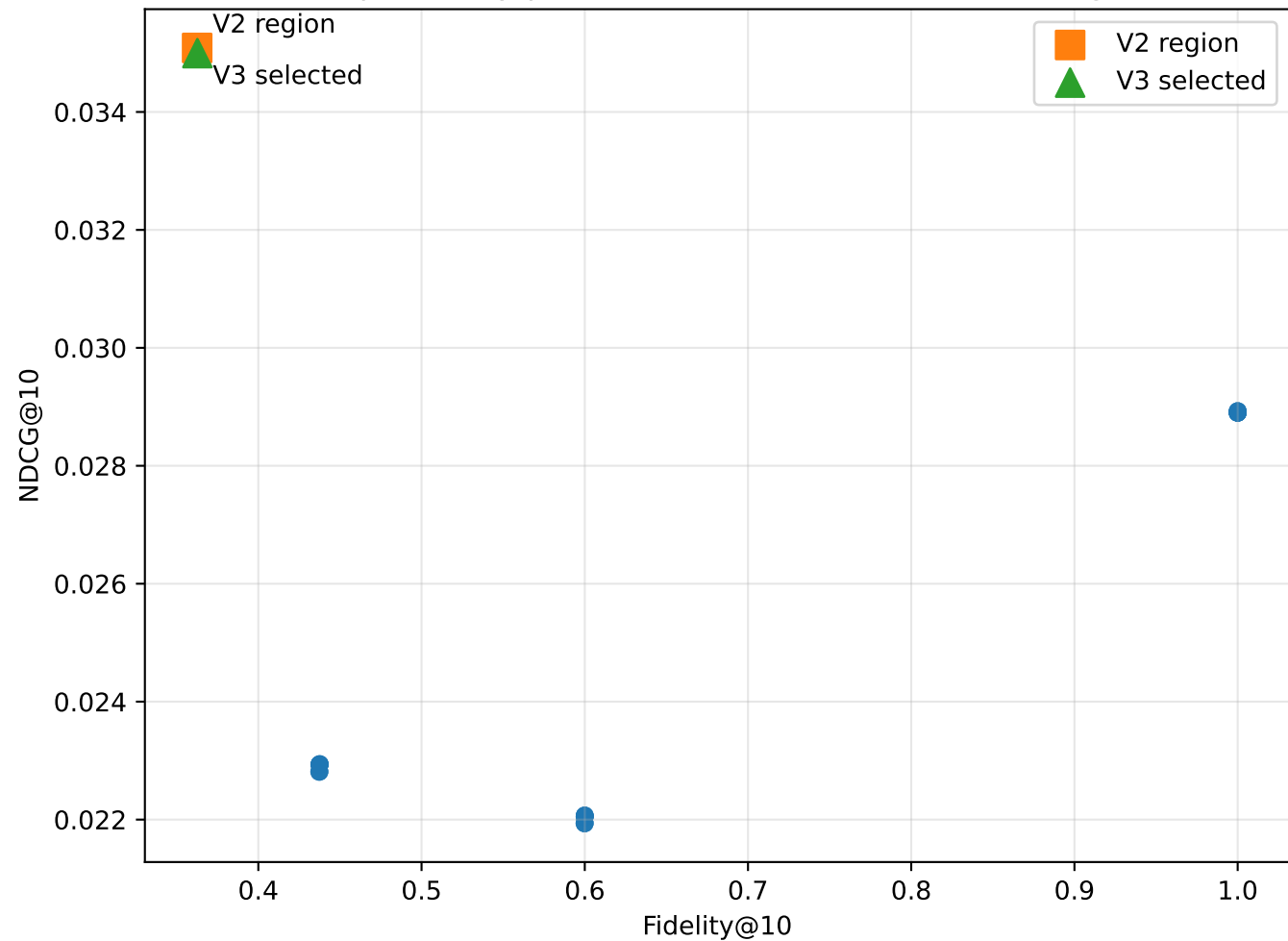
Interpretability-performance trade-off on validation grid
