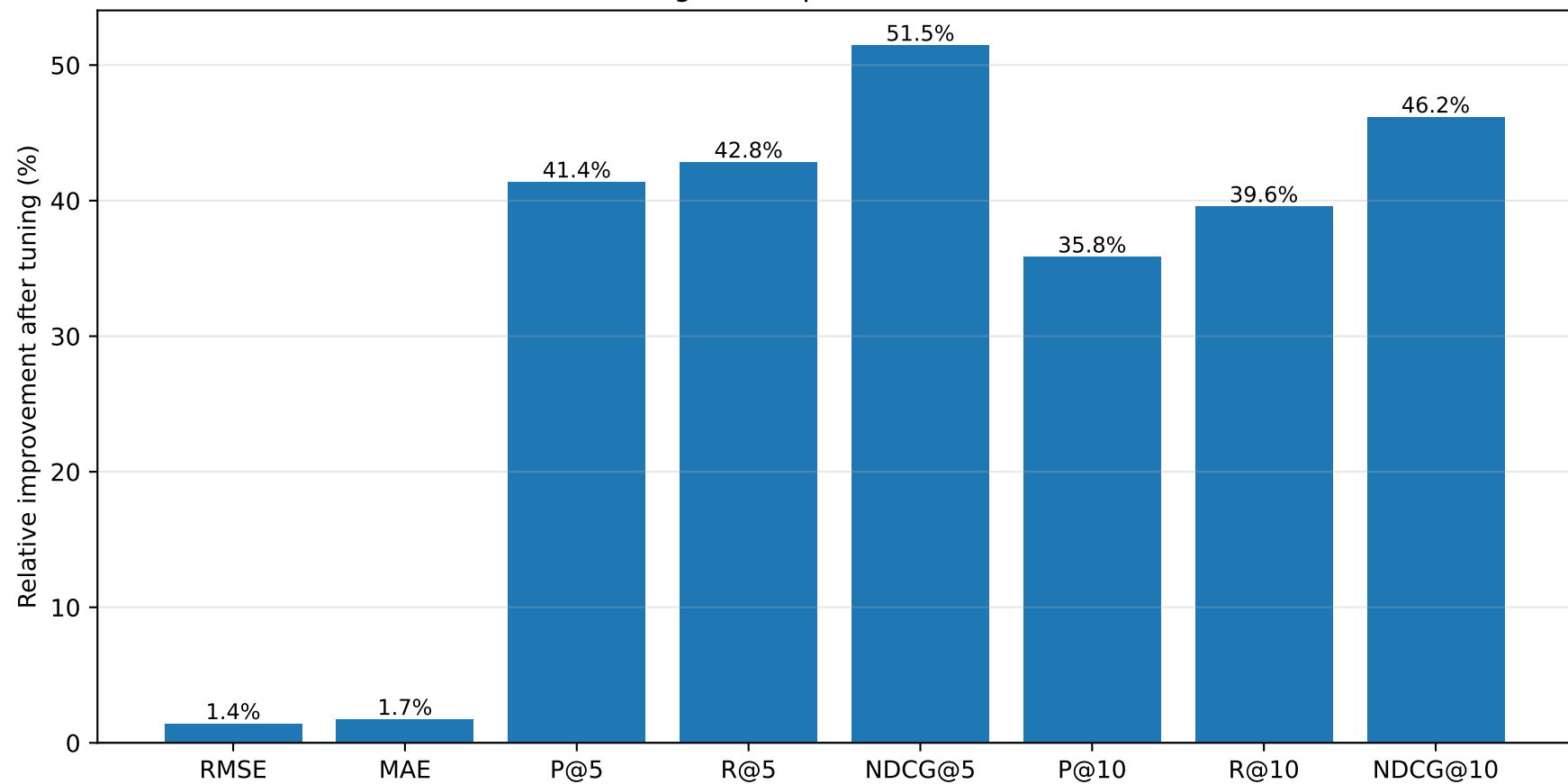
Effect of tuning on Coupled NMF for MovieLens 1M
