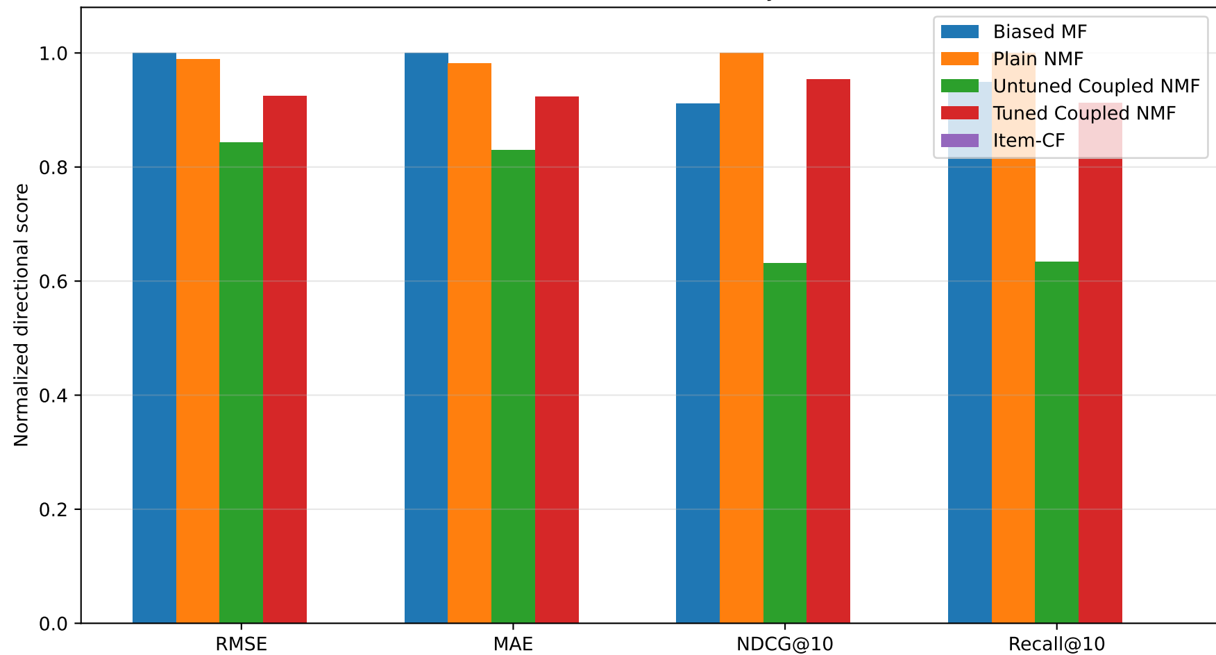
MovieLens 1M seed-42 secondary validation
