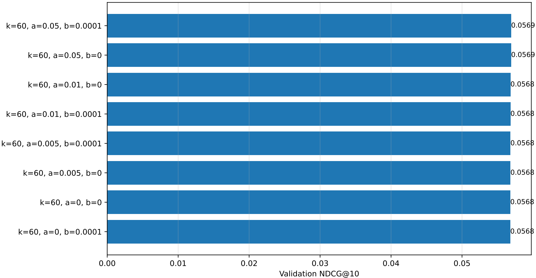
Top MovieLens 1M coupled-NMF tuning configurations
