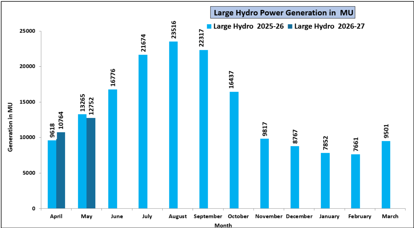
Figure 22: Month Wise Large Hydro Power Generation for the year 2026-27 & in year 2025-26.
