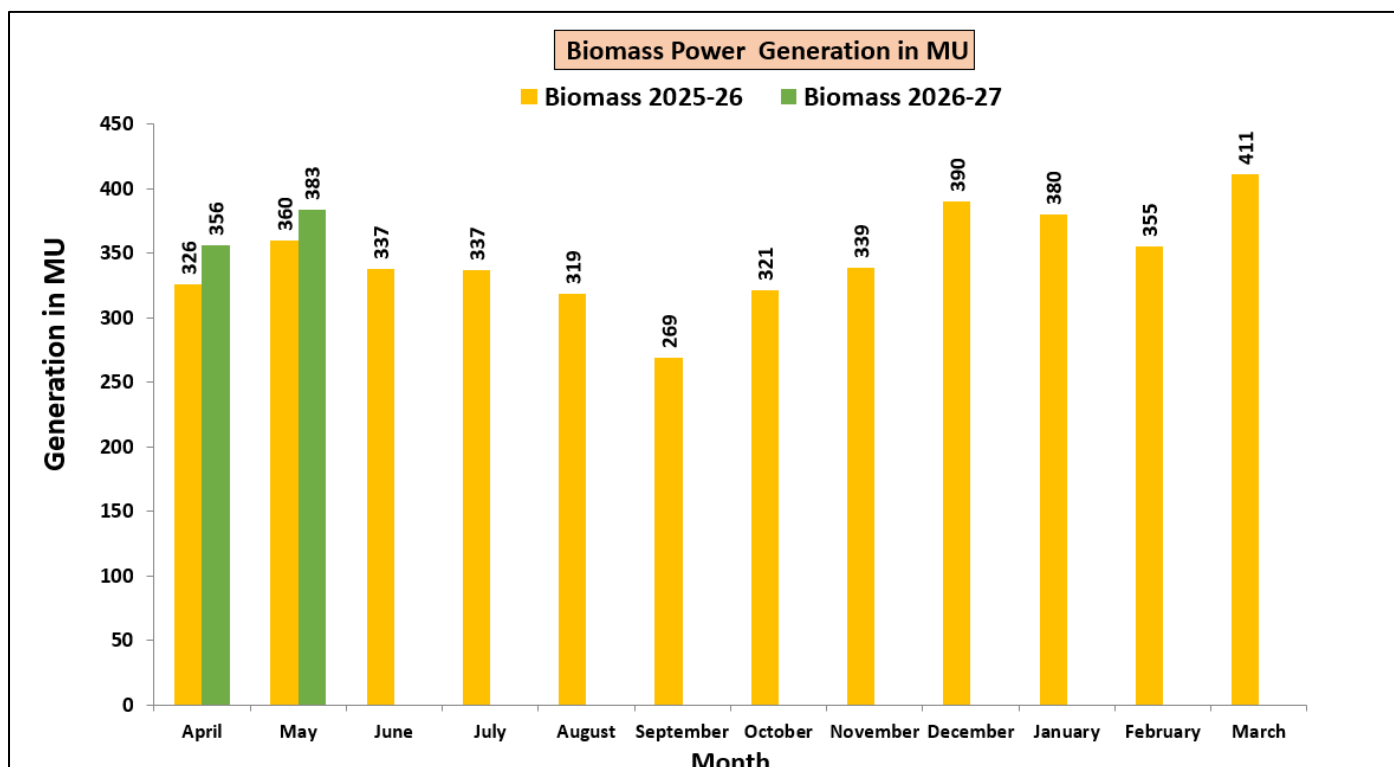
Figure 19: Month Wise Biomass Power Generation for the year 2026-27 & in year 2025-26.
