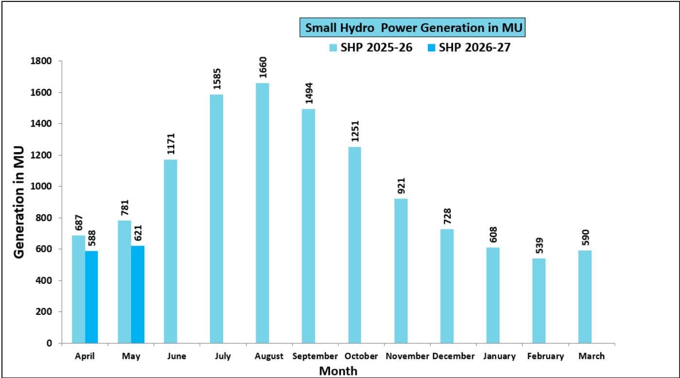
Figure 21: Month Wise Small Hydro Power Generation for the year 2026-27 & in year 2025-26.
