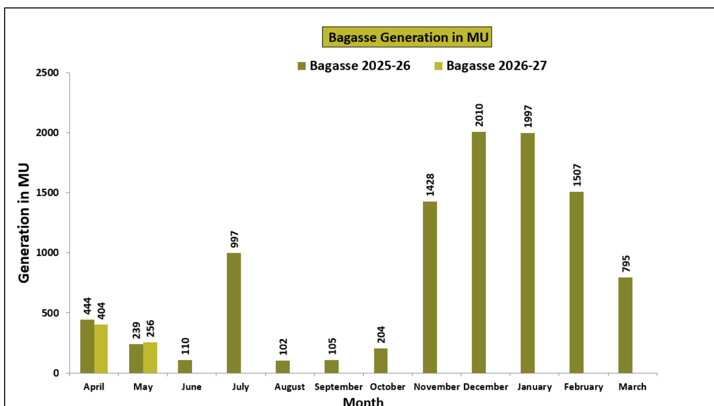
Figure 20: Month Wise Bagasse Power Generation for the year 2026-27 & in year 2025-26.
