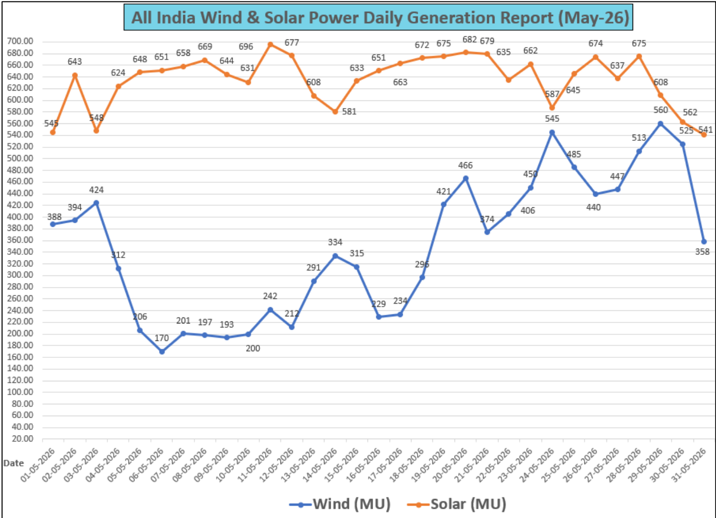
Figure 25: Daily solar and wind power generation in the month of May-2026
