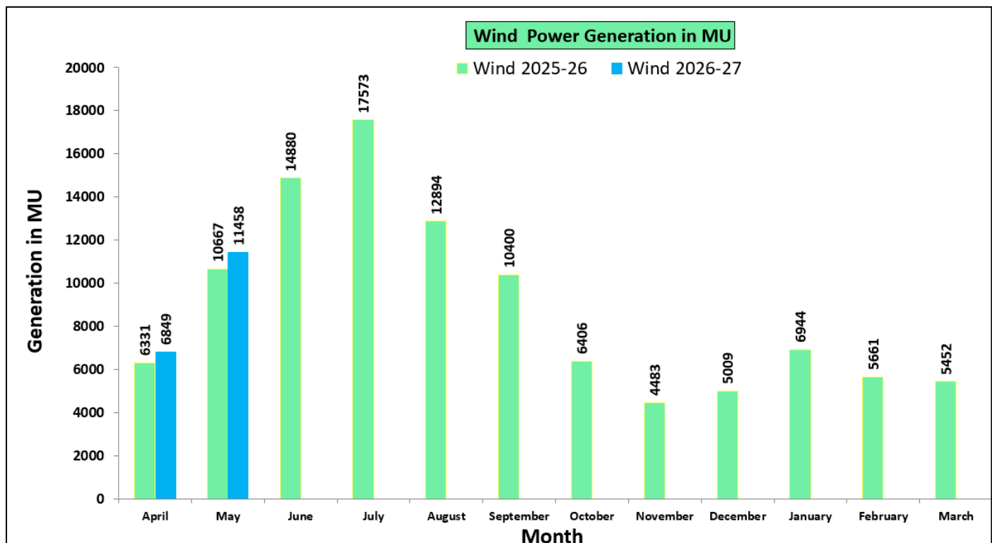
Figure 17: Month Wise Wind Power Generation for the year 2026-27 & in year 2025-26.
