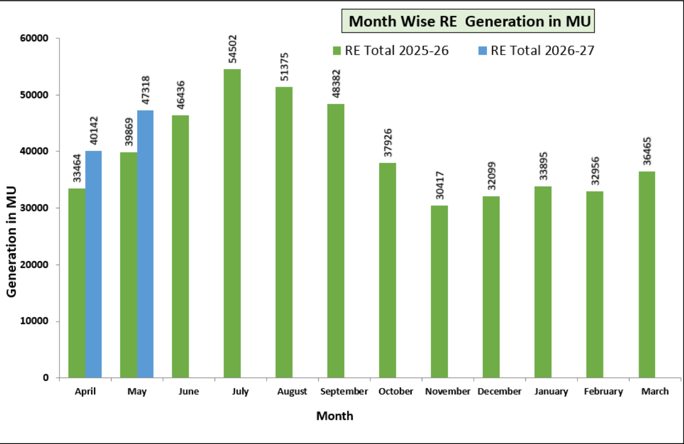
Figure 16: Comparison of Month Wise RE Generation in year 2026-27 & in year 2025-26.
