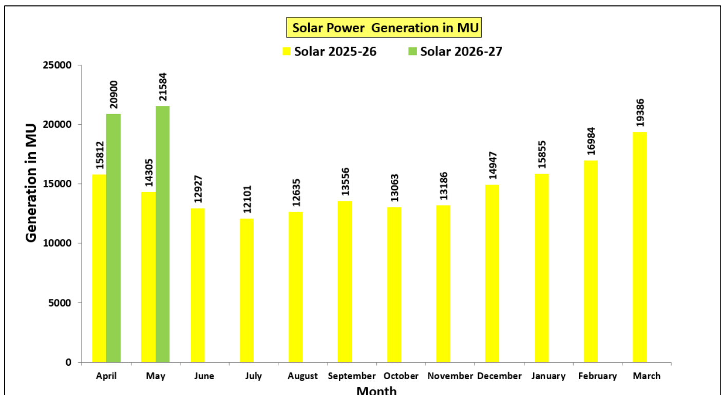
Figure 18: Month Wise Solar Power Generation for the year 2026-27 & in year 2025-26.
