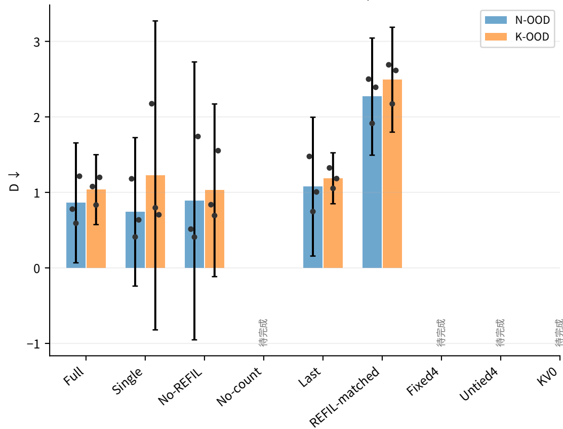
c. Relation probes: 50v50 K2 confirmation
