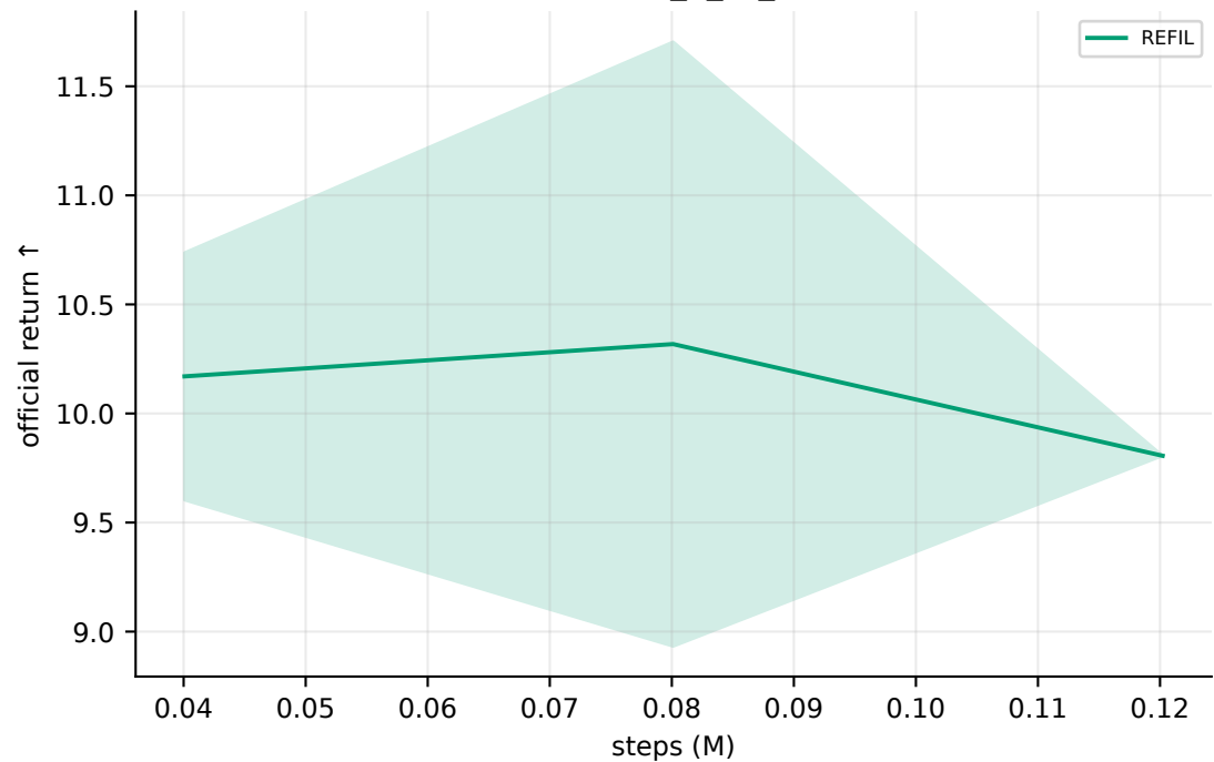
protoss_8_vs_8
