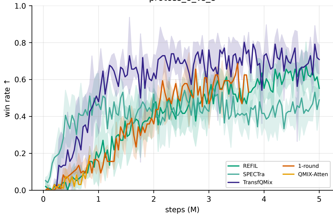
protoss_8_vs_8
