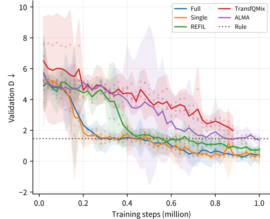
d. SMACv2 learning
