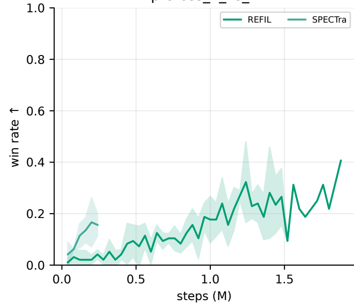
protoss_4_vs_4
