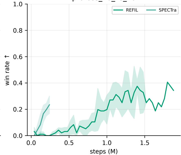
protoss_10_vs_10
