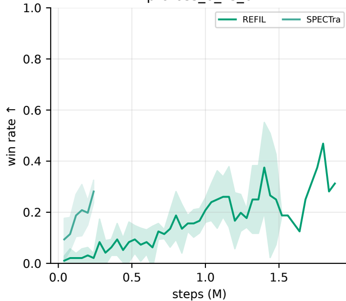
protoss_6_vs_6
