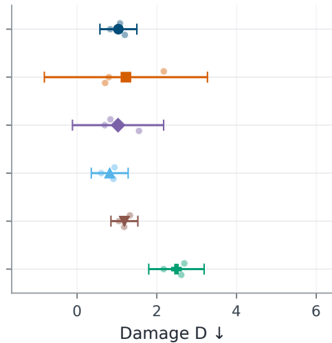
(b) K-OOD
