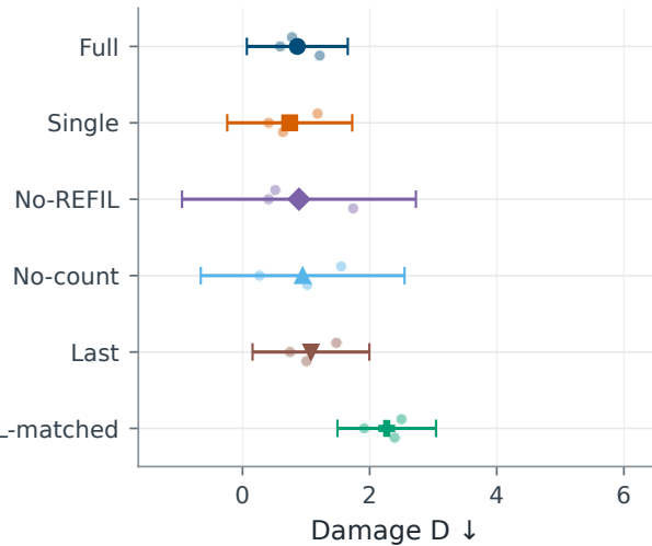
(a) N-OOD
