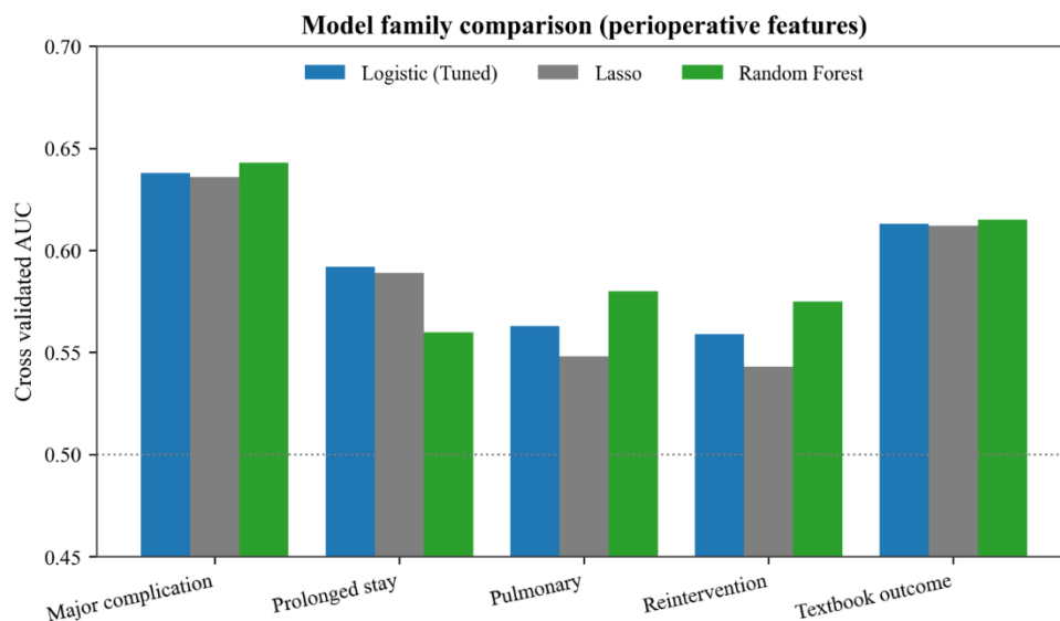
Figure 4.4. Discrimination of the logistic model, the lasso, and the random forest on the perioperative features.
