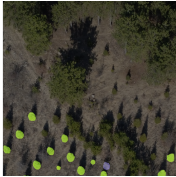
Generated masks
