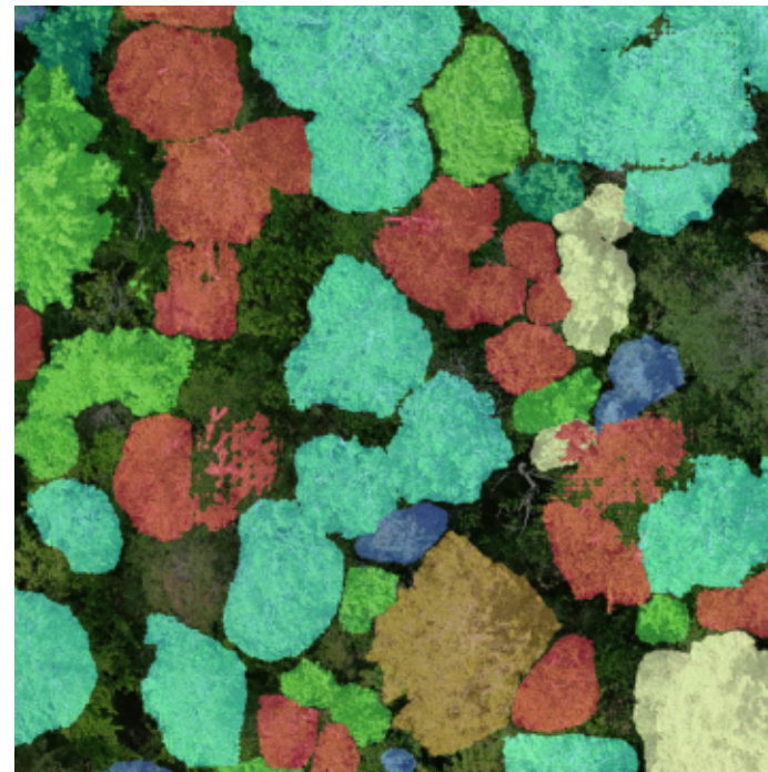
Generated masks
