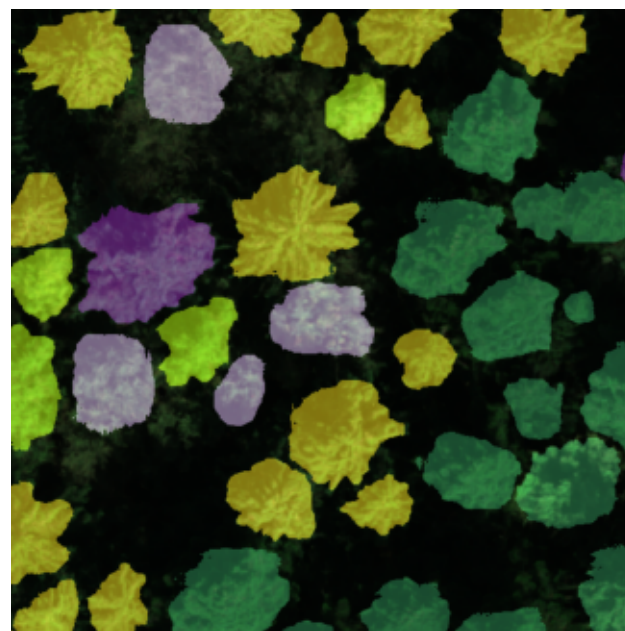
Generated masks
