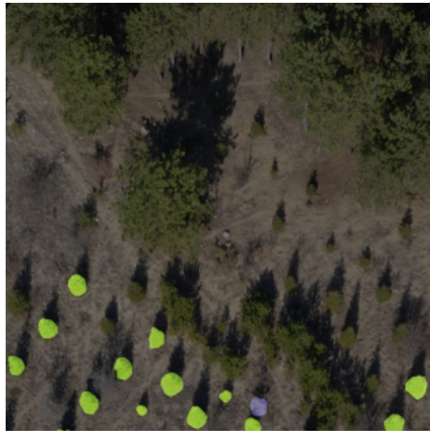
Real masks
