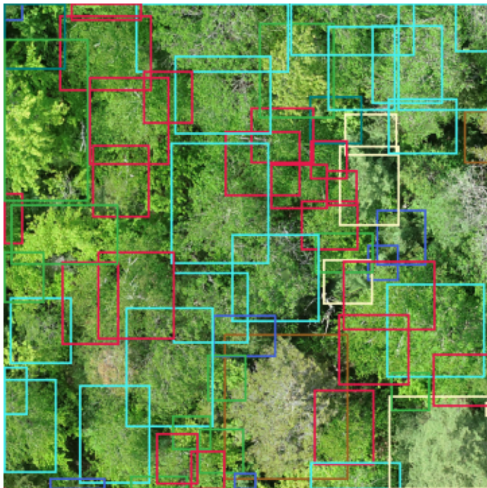
Bounding boxes
