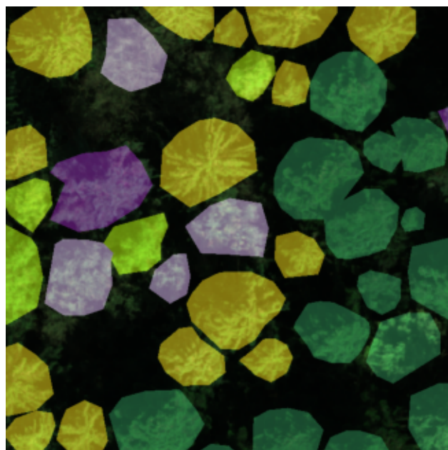
Real masks
