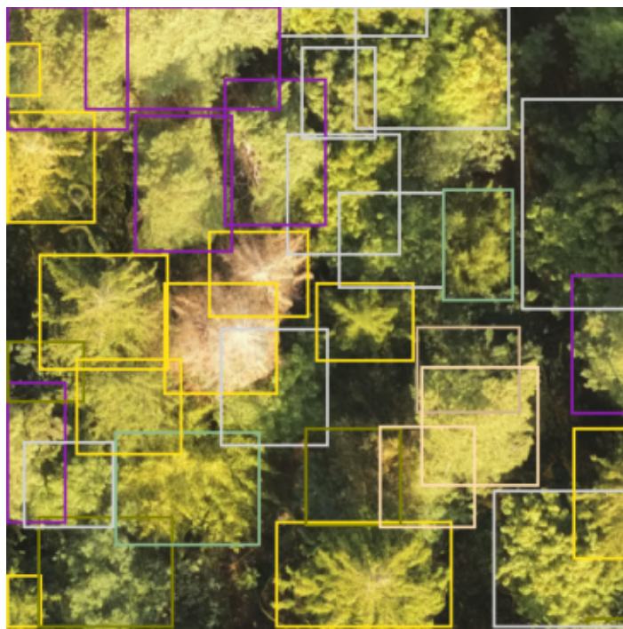
Bounding boxes
