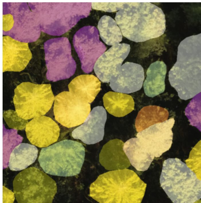
Real masks
