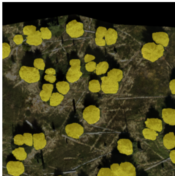
Generated masks
