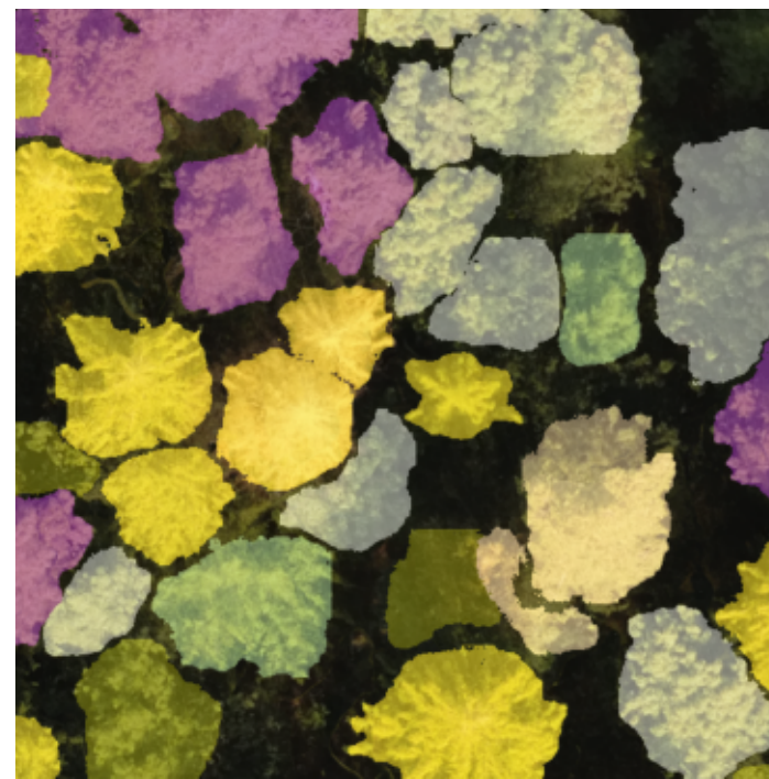
Generated masks
