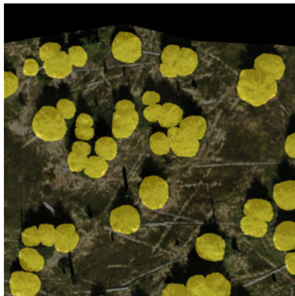
Real masks
