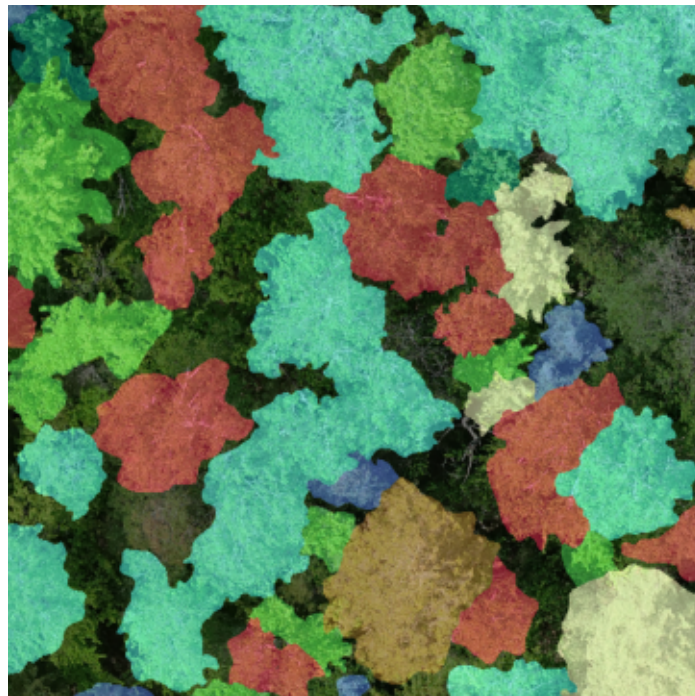
Real masks
