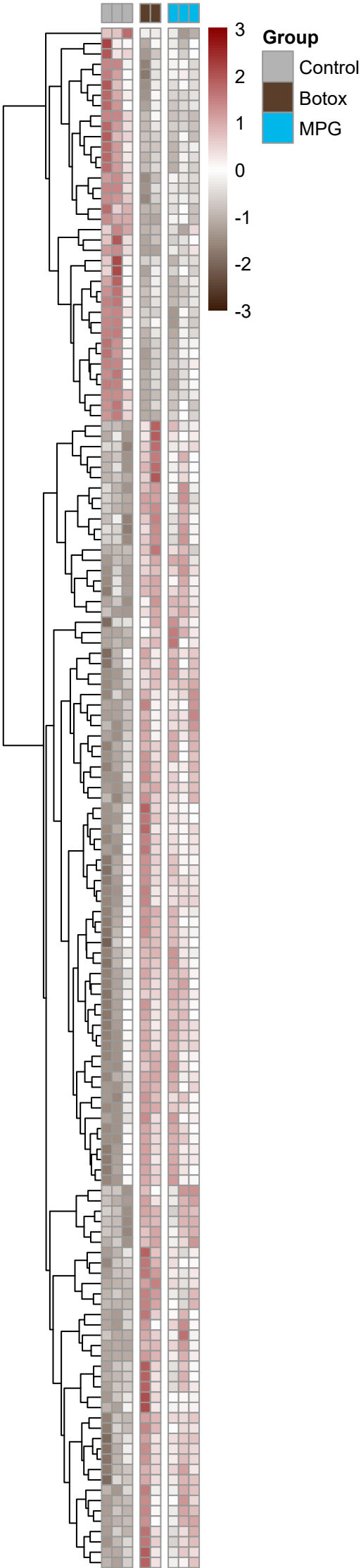
PR-DV_1.5x_Aver - all DEGs
