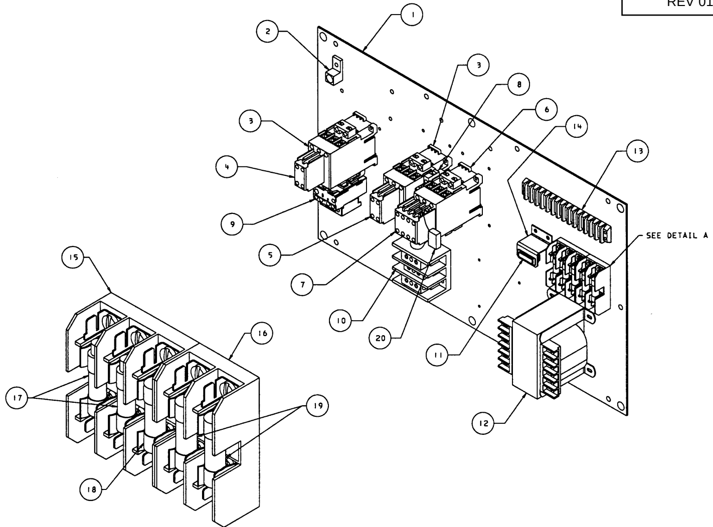
DETAIL A
