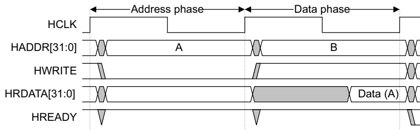
Figure 3-1 Read transfer
