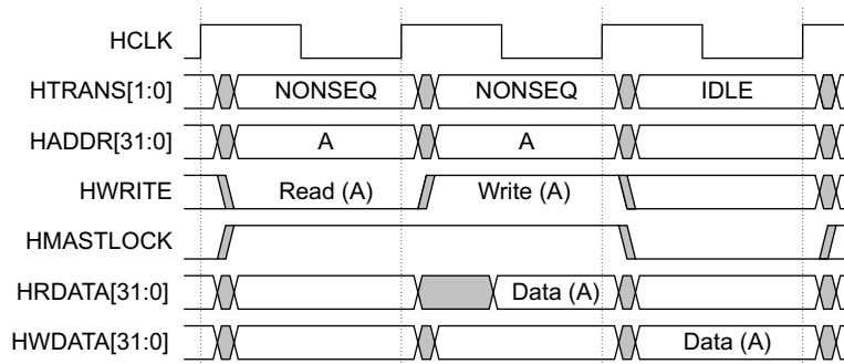
Figure 3-7 Locked transfer
