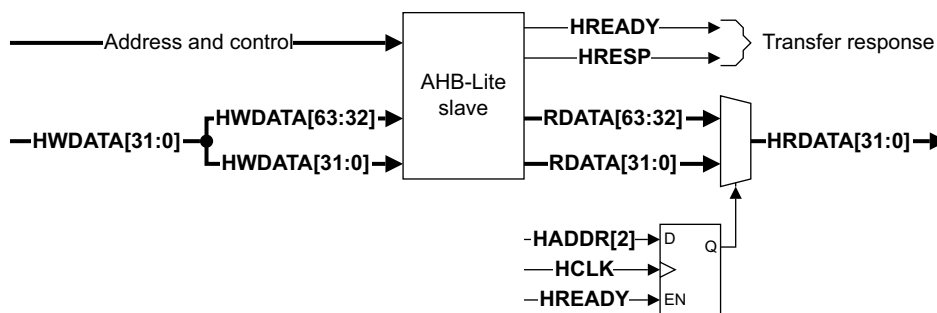
Figure 6-2 Wide slave on a narrow bus
