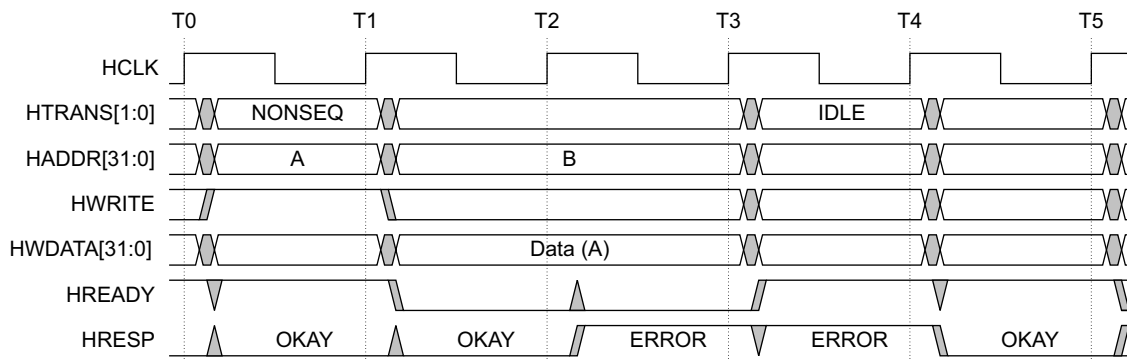
Figure 5-1 ERROR response
