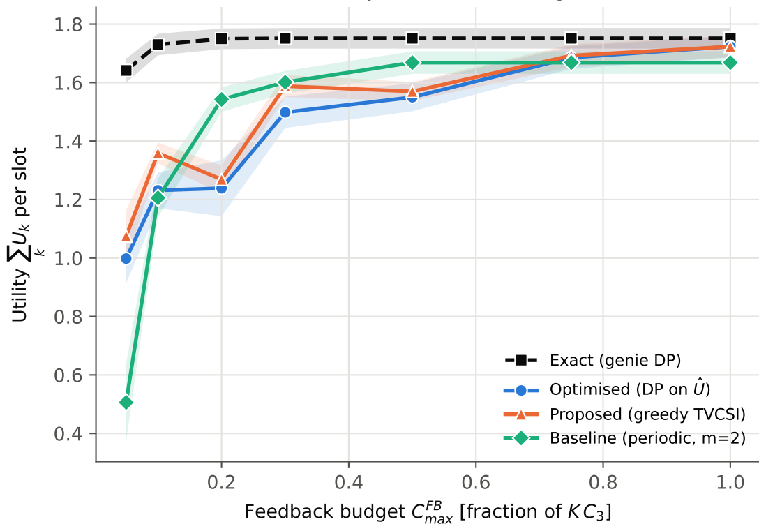
Task utility vs feedback budget
