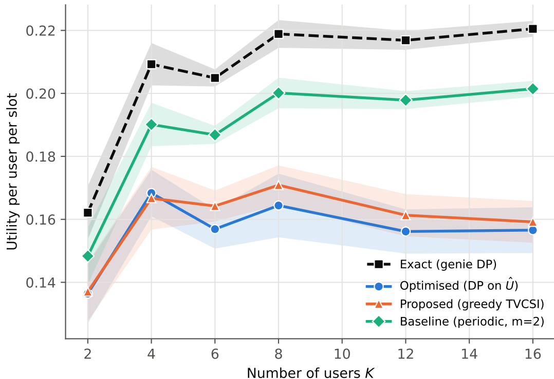
Per-user task utility vs number of users
