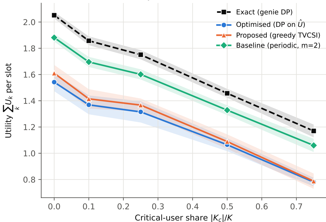
Task utility vs share of critical users
