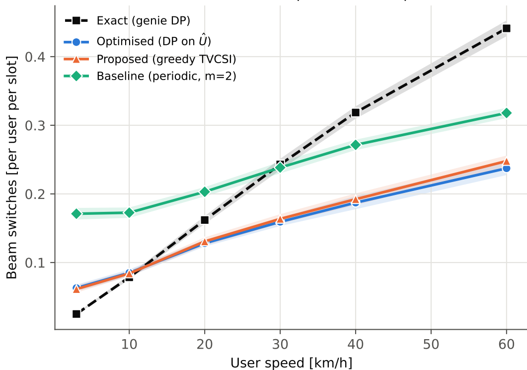
Beam-switch rate (Eq. 38) vs user speed
