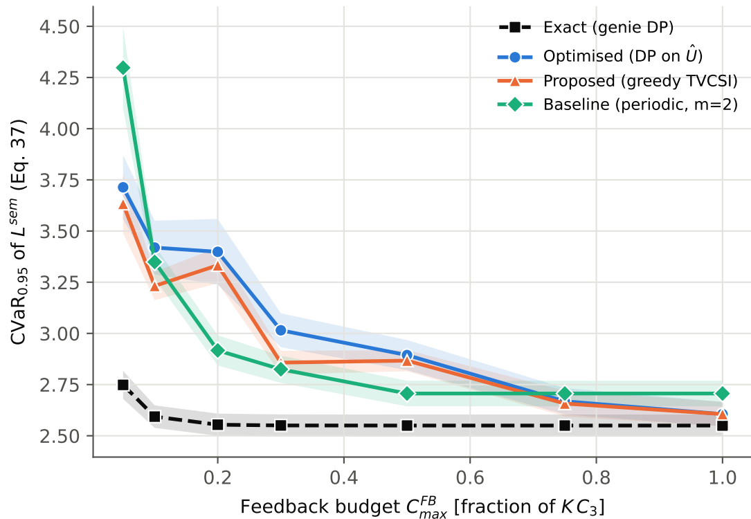
Tail semantic loss vs feedback budget
