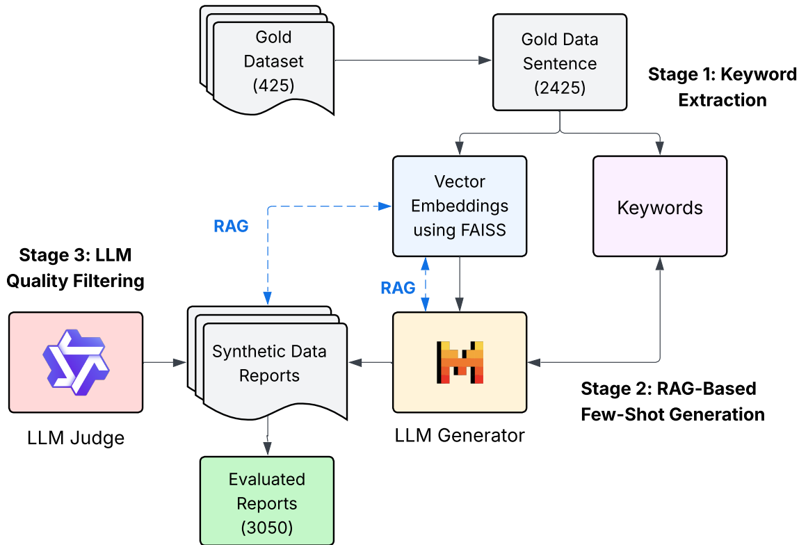
Synthetic Data Generation & Evaluation Pipeline
