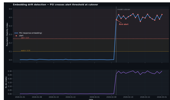
Drift detection - PSI crosses the alert threshold exactly at the model cutover
