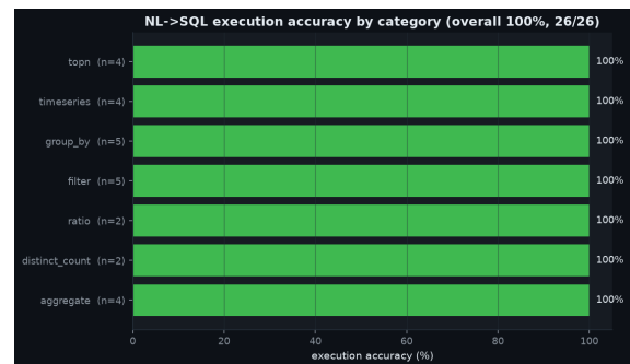
NL->SQL execution accuracy by category
