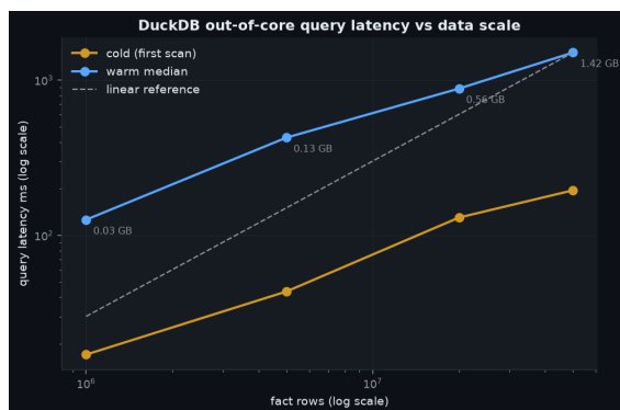
Query latency vs data scale (log-log)
