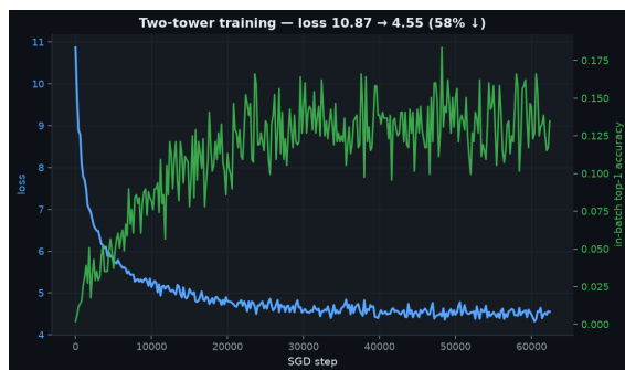
Two-tower training curve
