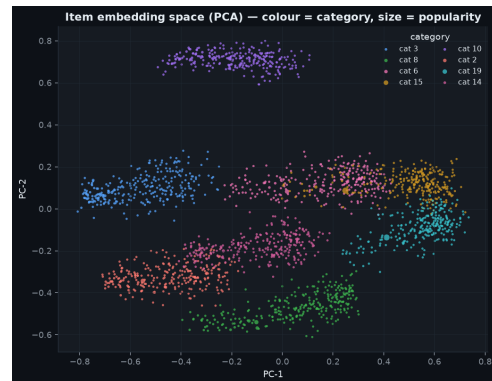
Item embedding space (PCA), coloured by category
