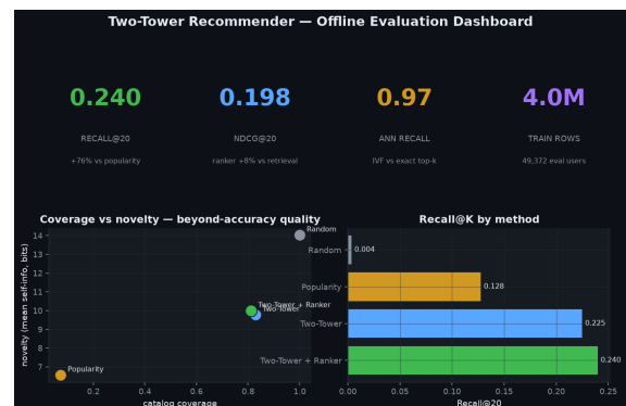
Offline evaluation dashboard
