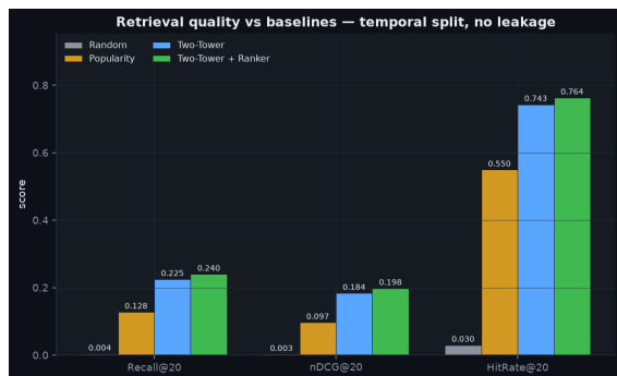
Retrieval quality vs baselines
