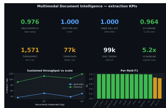
Extraction KPIs + throughput scaling
