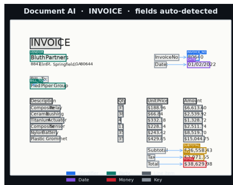
Detected fields on a rendered document (the product view)
