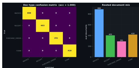
Document-type router: confusion matrix + routed mix
