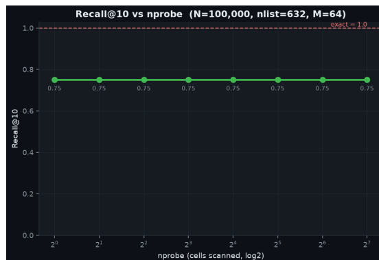
Recall@10 vs nprobe (the accuracy dial)
