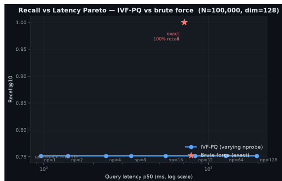
Recall vs Latency Pareto - IVF-PQ vs brute force
