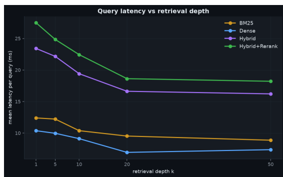
Query latency vs retrieval depth
