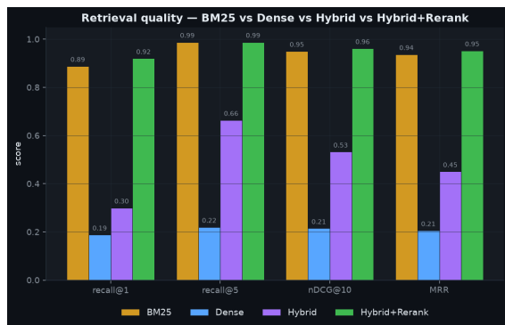
Retrieval quality - 4 methods compared
