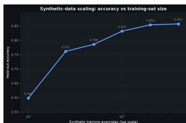
Synthetic-data scaling
