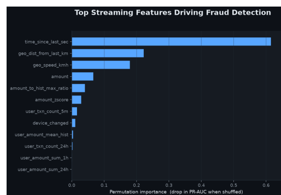
Permutation feature importance
