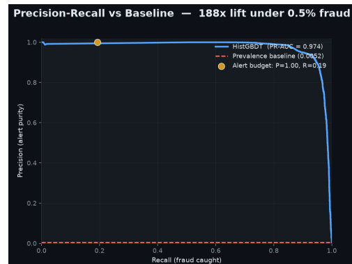
Precision-Recall vs baseline
