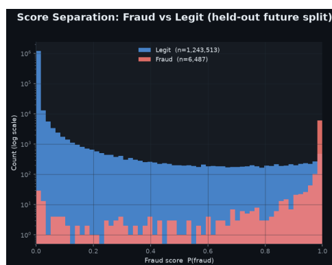
Score distribution - fraud vs legit
