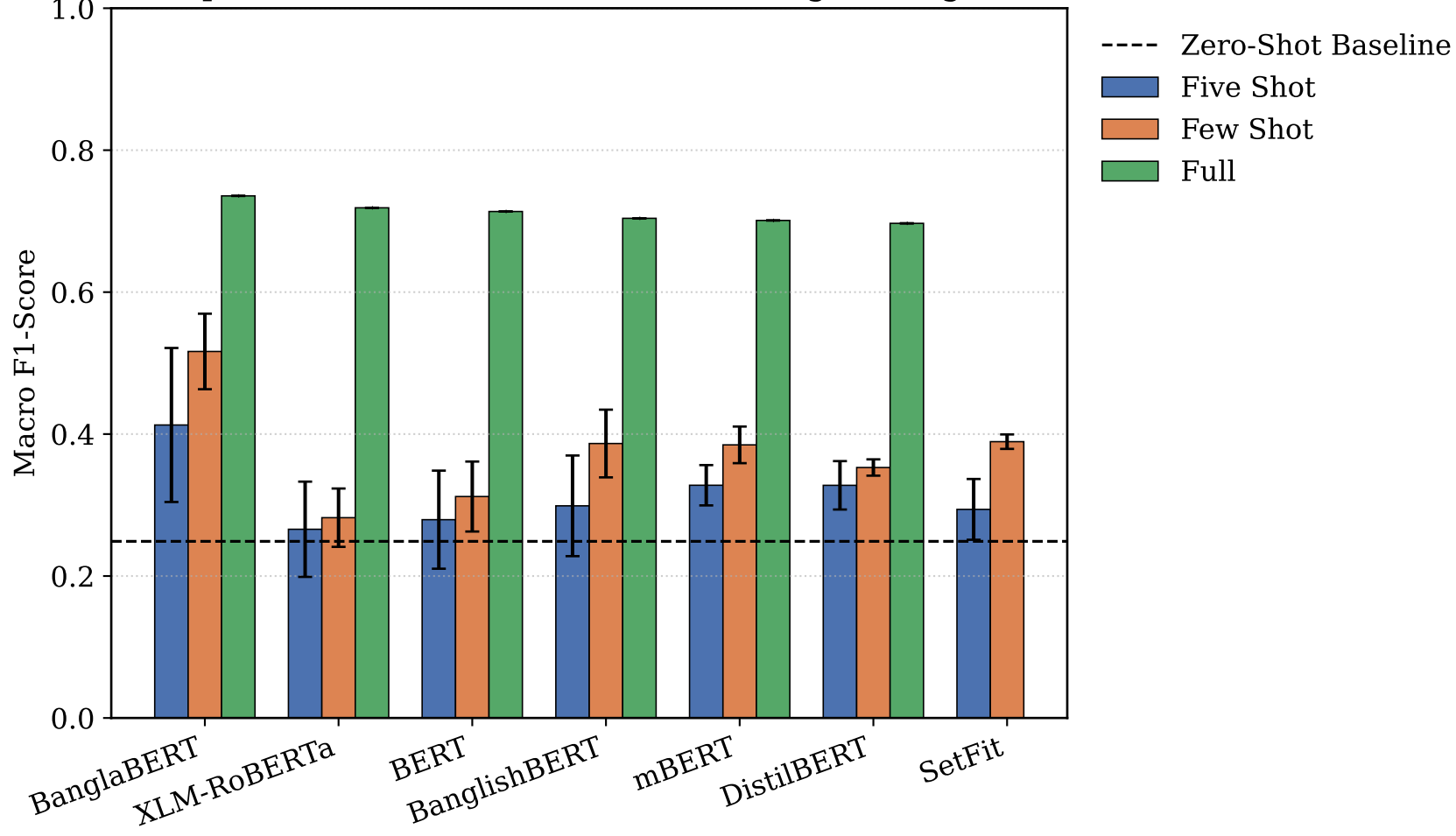
Macro-F1 Comparison Across Models and Learning Settings on BnSentMix
