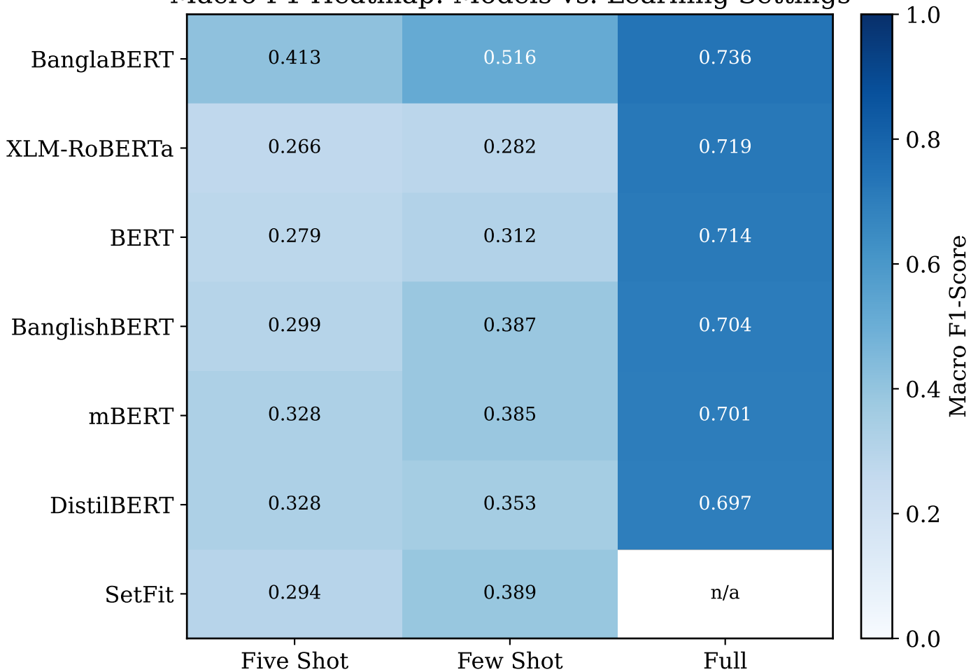
Macro-F1 Heatmap: Models vs. Learning Settings
