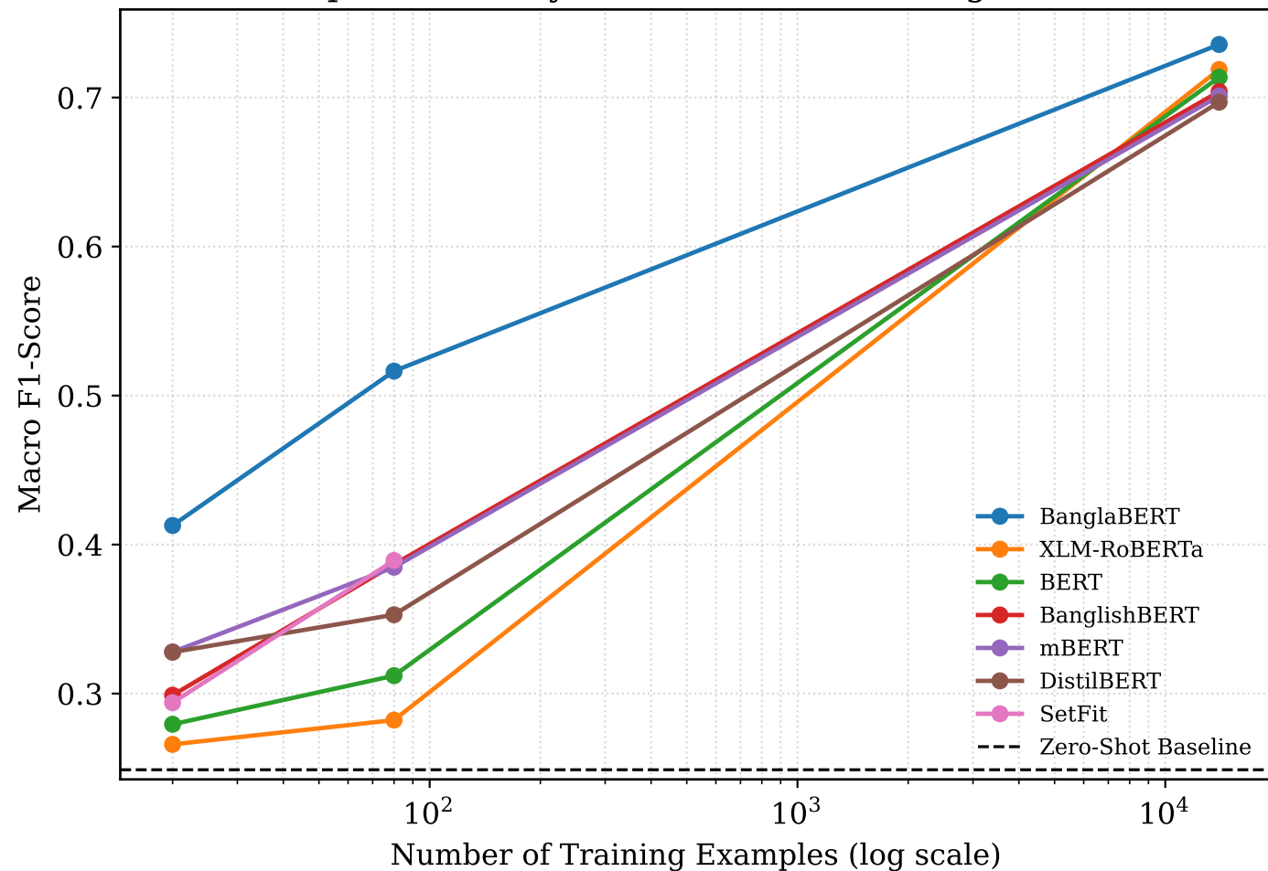
Sample Efficiency: Macro-F1 vs. Training Set Size
