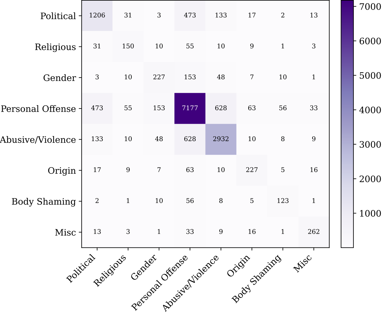
Co-occurrence of Multi-Label Hate Targets (re-derived from loaded data)
