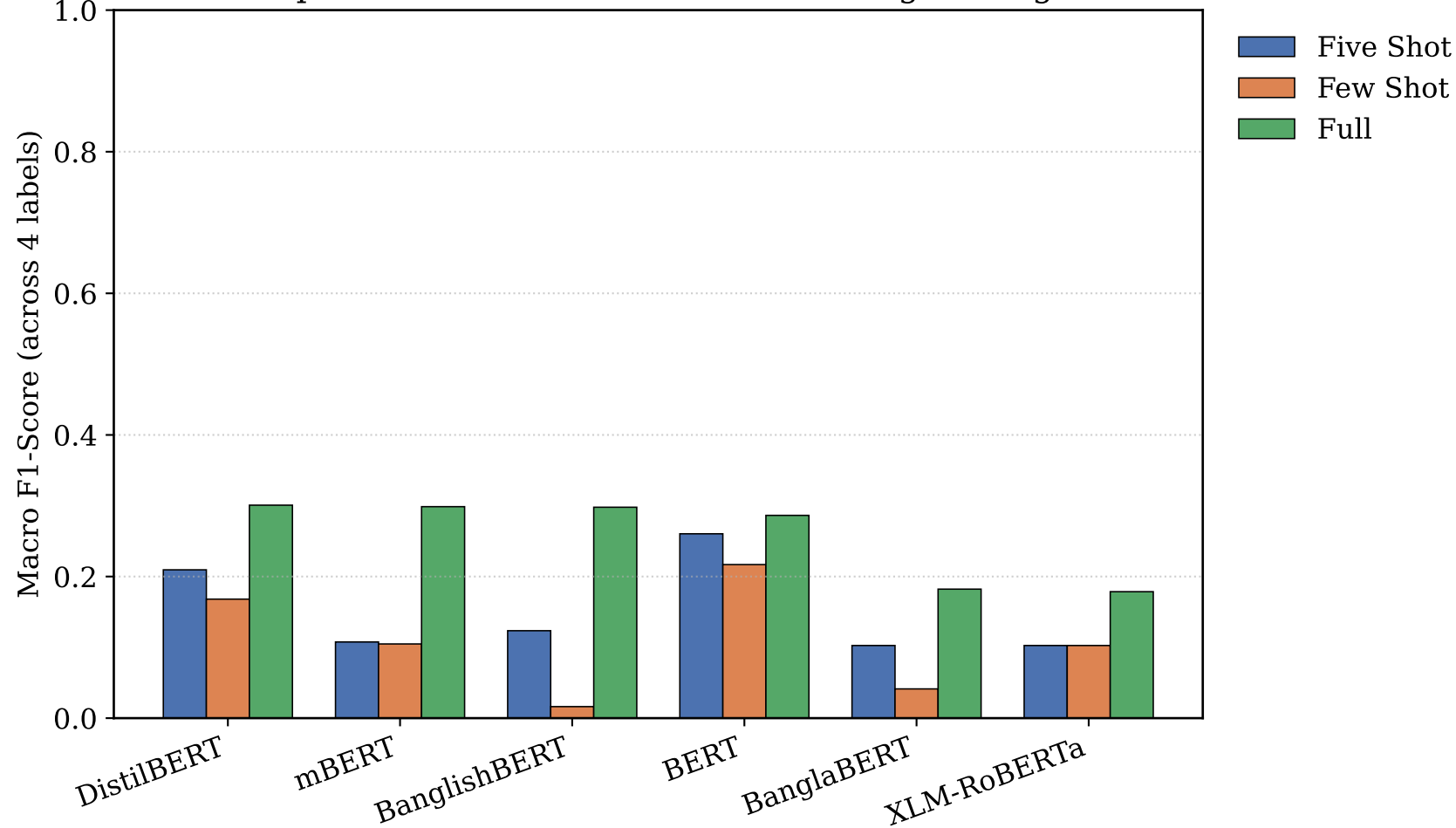
Macro-F1 Comparison Across Models and Learning Settings on MixSarc
