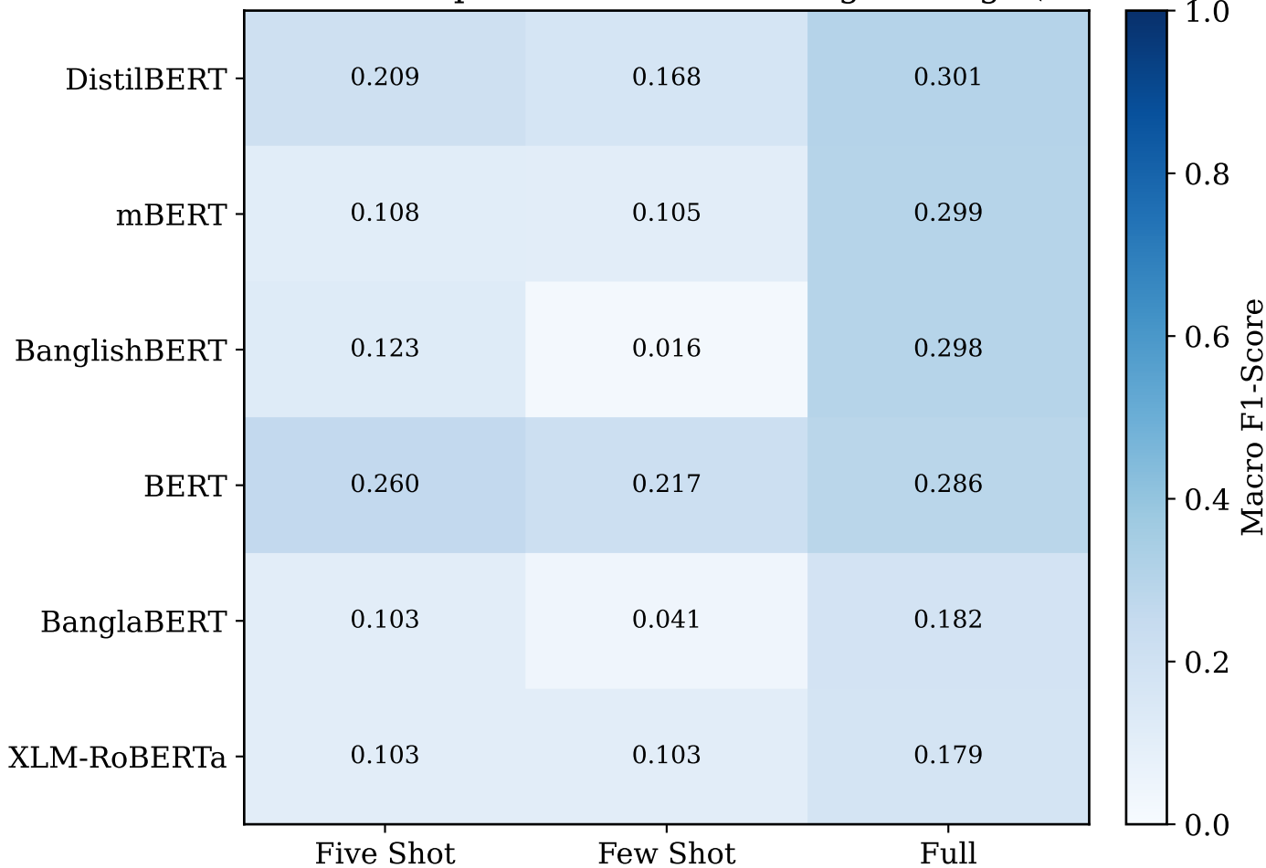
Macro-F1 Heatmap: Models vs. Learning Settings (MixSarc)
