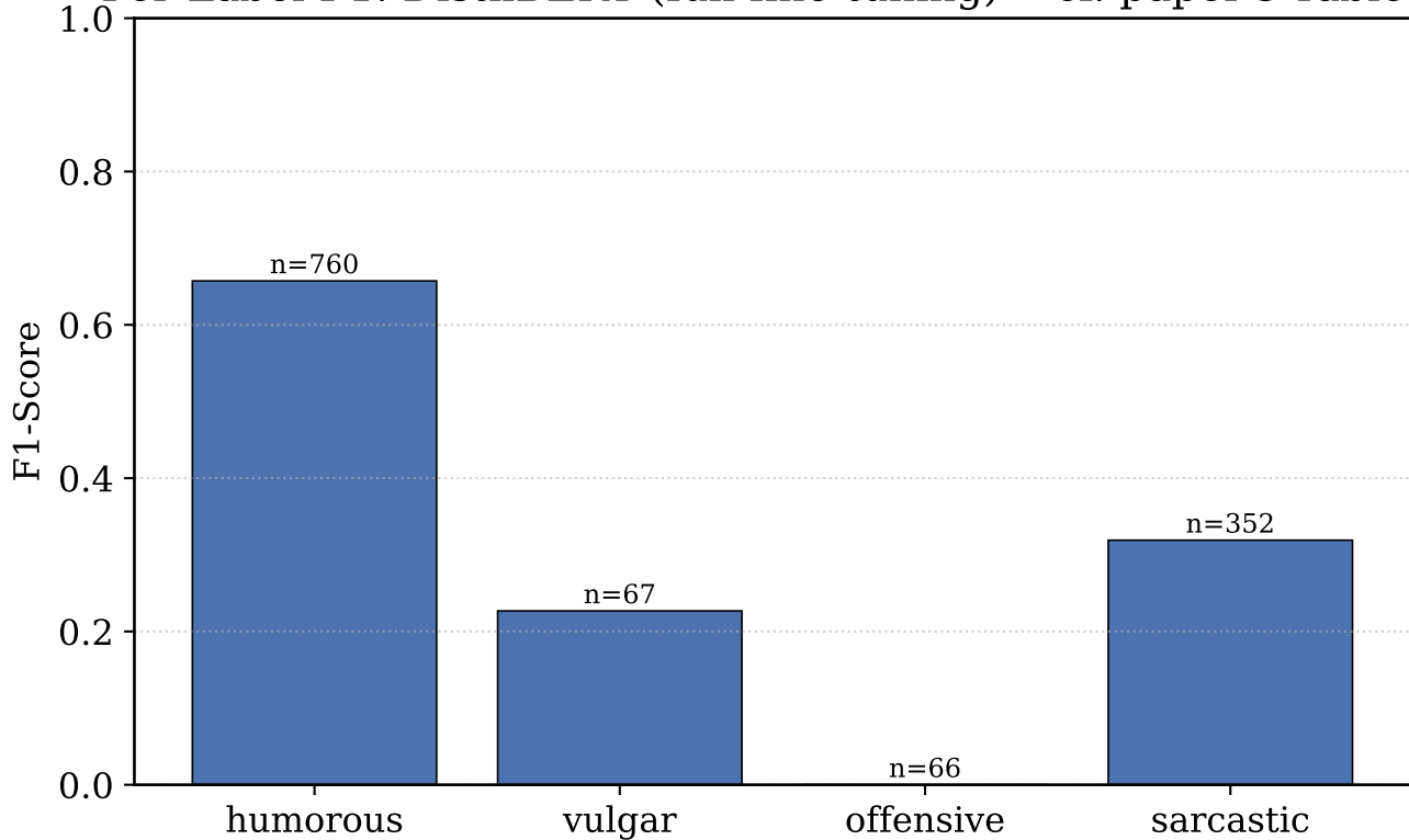
Per-Label F1: DistilBERT (full fine-tuning) -- cf. paper's Table 5
