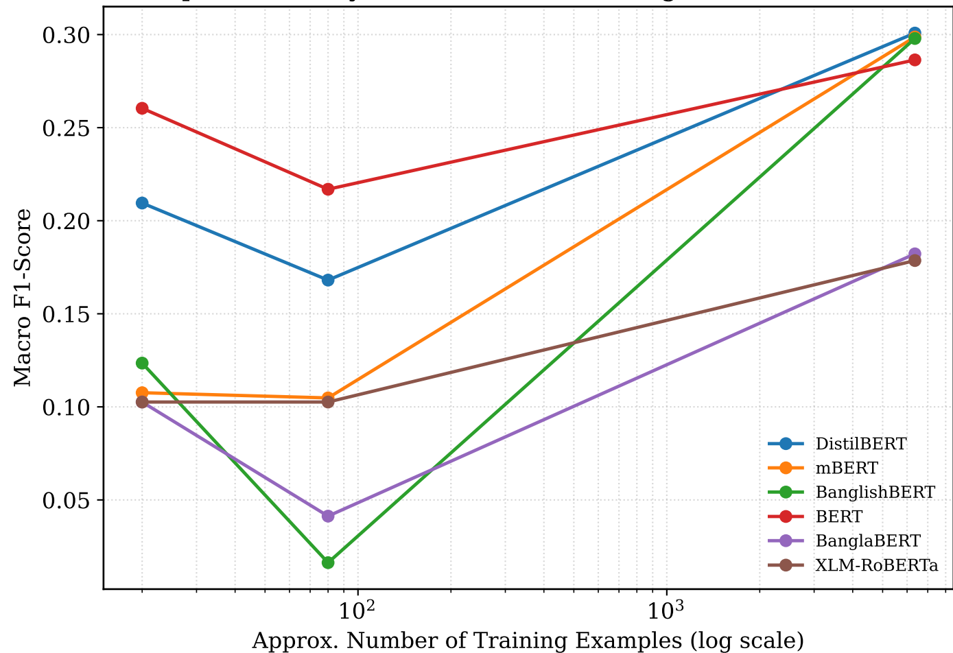
Sample Efficiency: Macro-F1 vs. Training Set Size (MixSarc)
